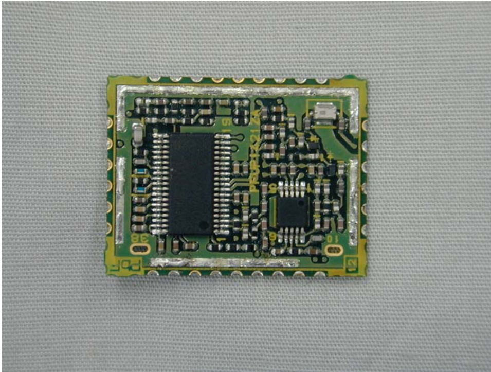
RF module for both base unit and handset (mount inside the shield case)
