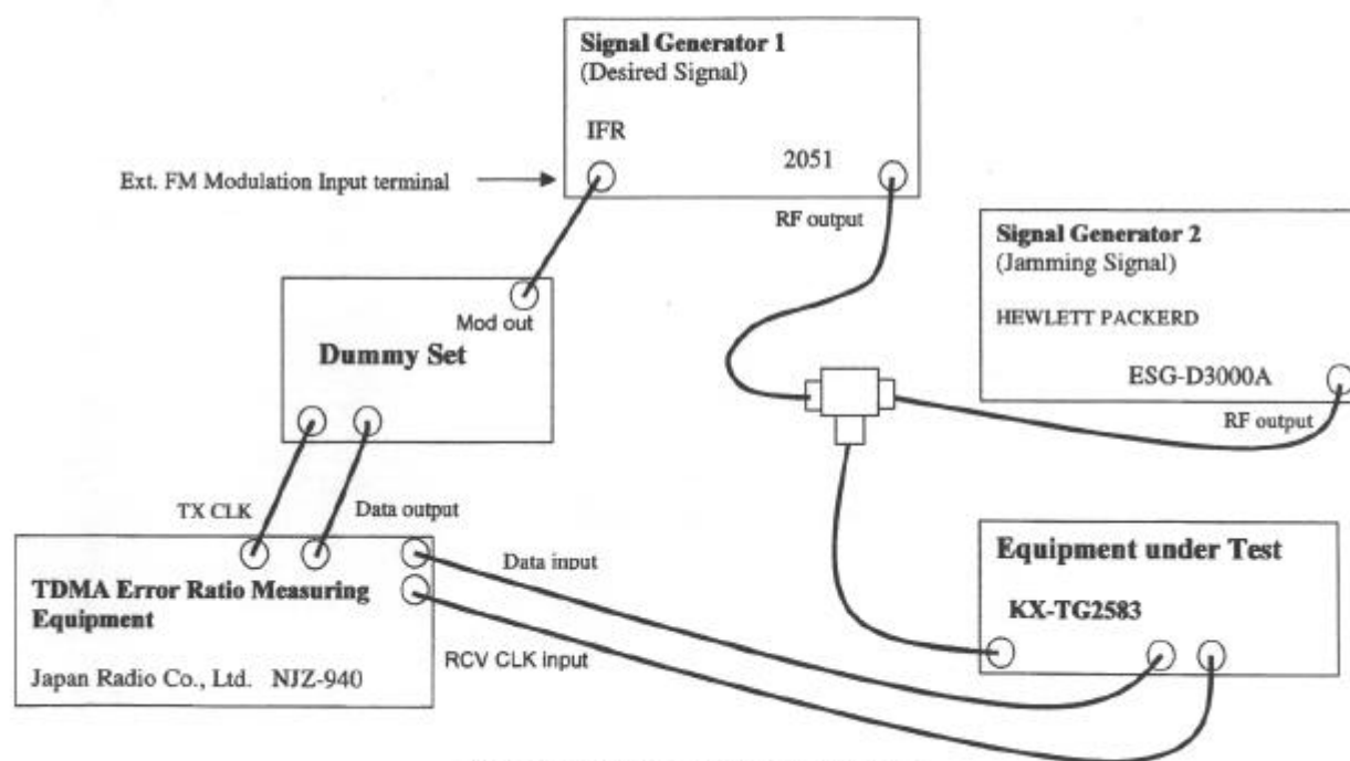
Figure 1: Processing Gain Test Setup
