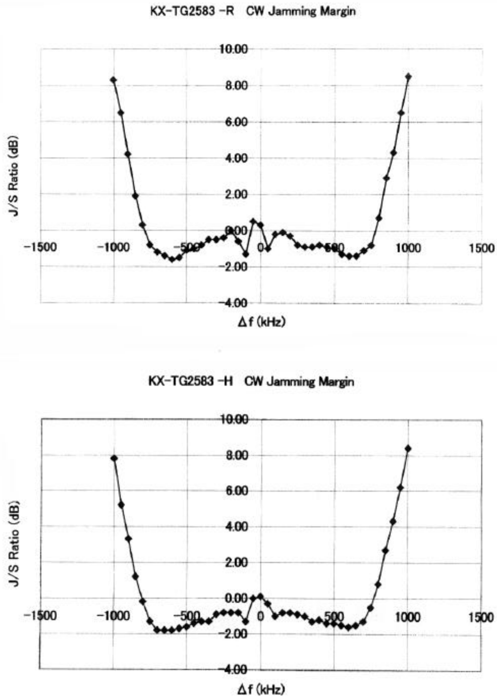
Figure 3: Test Results of Jamming Margin
