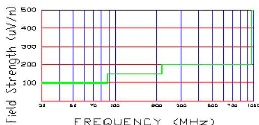
Figure 10. Restrictd band harmonics and spurious limits.
