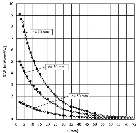
Figure 5. E-Field and Temperature measurements at 900MHz [5]
