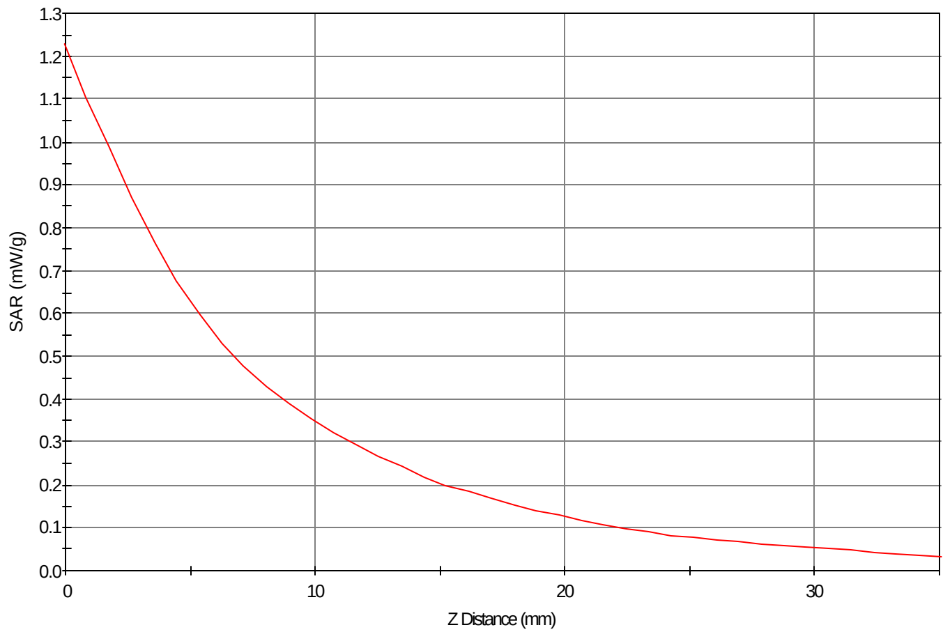
SAR - Z Axis at Hotspot x:24.0 y:-1.0
