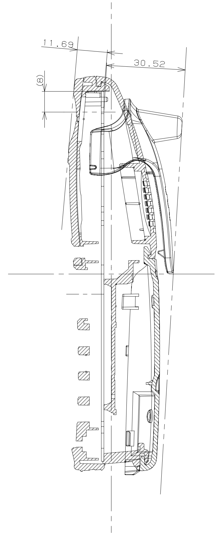
KX-TGA546/TGA551 1.4 color
