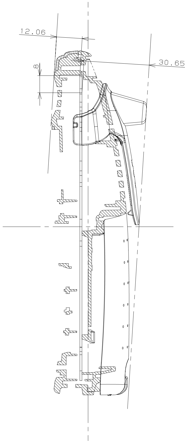
KX-TGA548/TGA549 Shock
