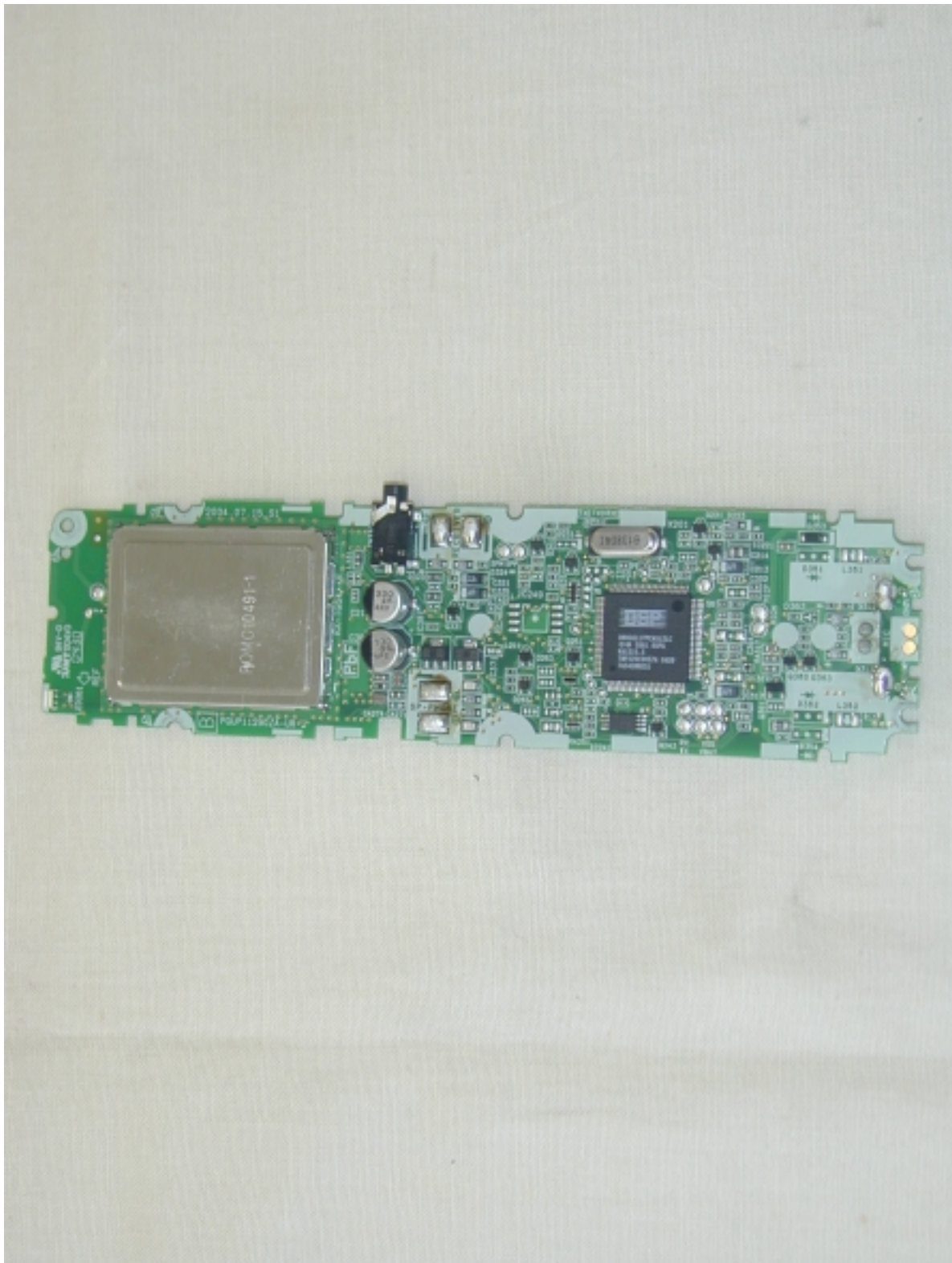
Portable Unit, KX-TGA549 (Printed Circuit Board)
