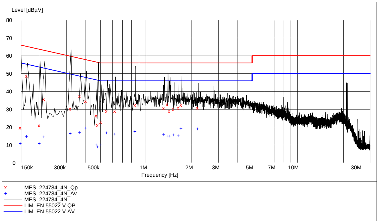
PNLV226(FW), Off-Hook Mode (Plot shows worst case of Phase L1 and N)
