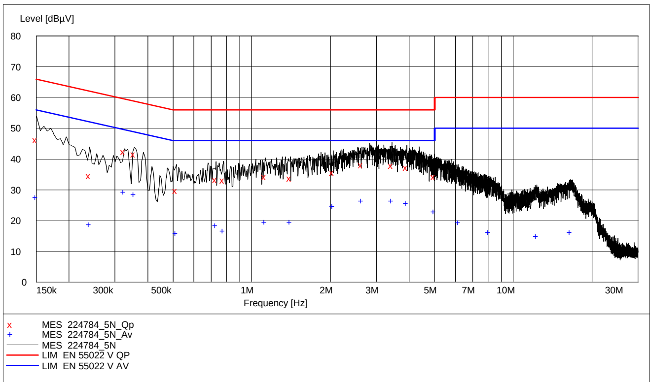
PNLV226(UC), Charger Mode (Plot shows worst case of Phase L1 and N)
