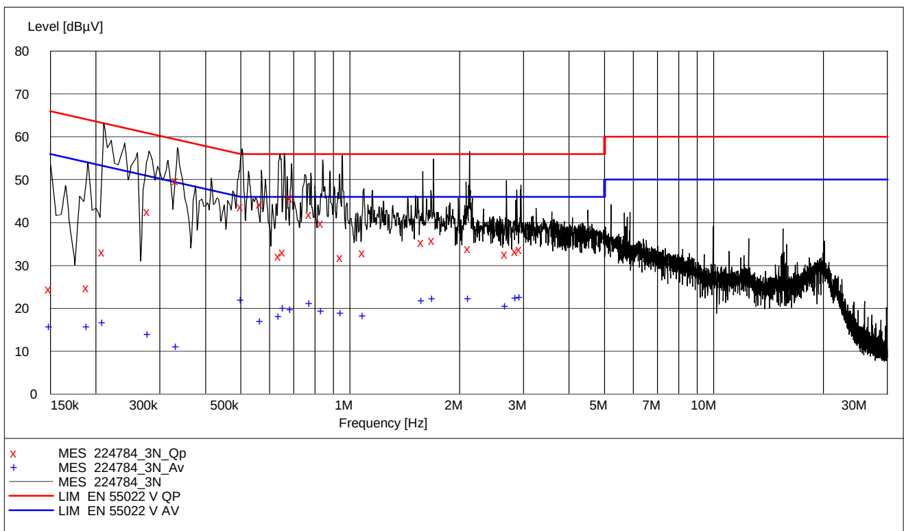
PNLV226(FW), Charger Mode (Plot shows worst case of Phase L1 and N)
