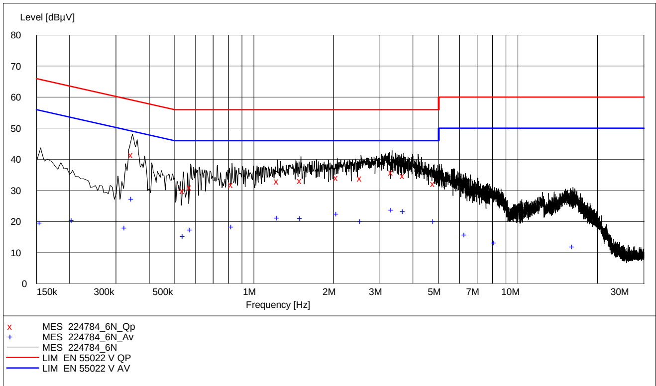
PNLV226(UC), Off-Hook Mode (Plot shows worst case of Phase L1 and N)
