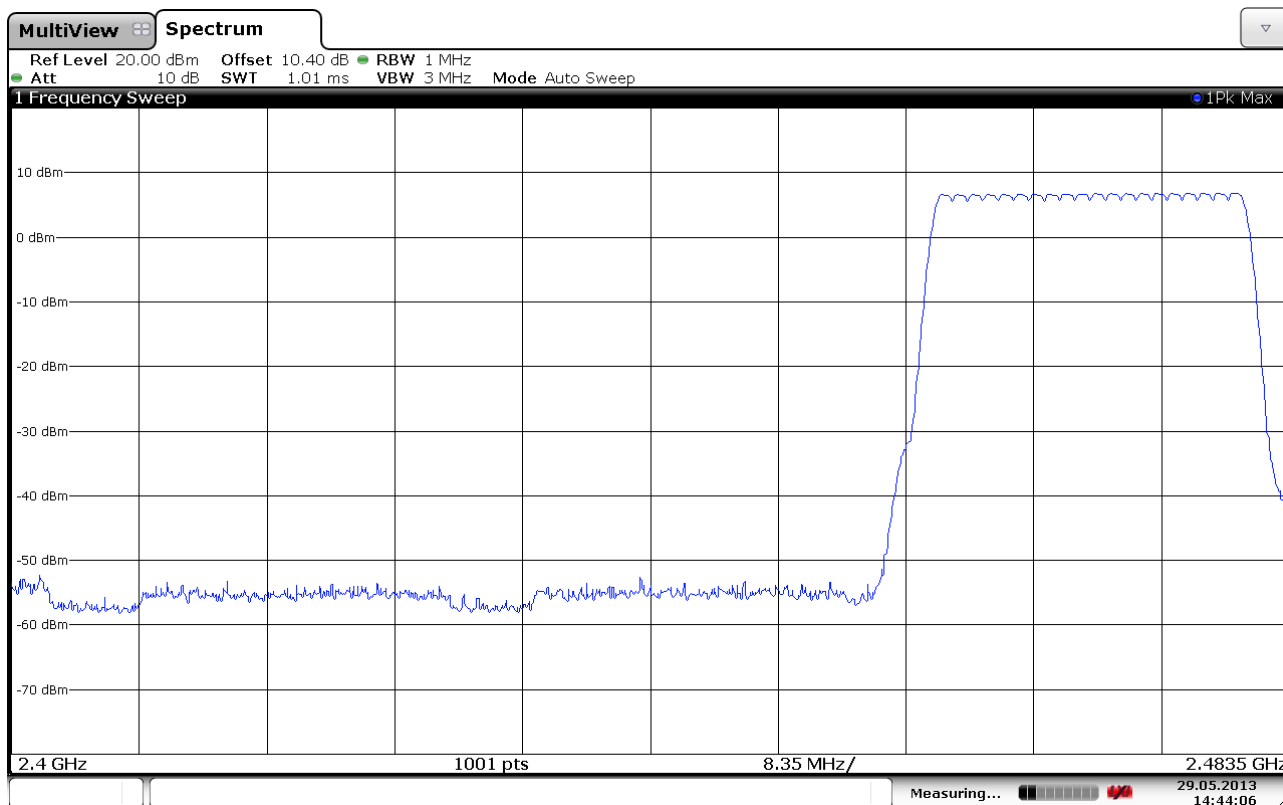
RF Channels in Use, 20 Channels, Upper
