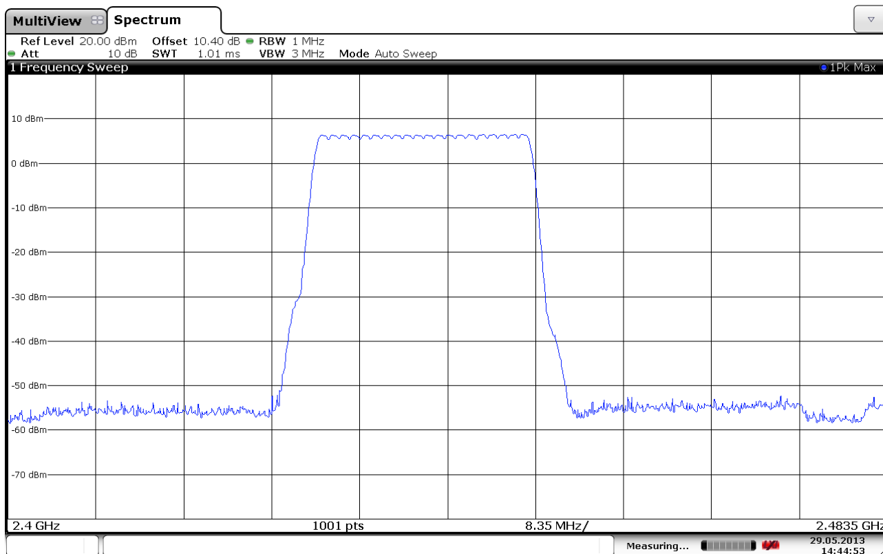
RF Channels in Use, 20 Channels, Middle
