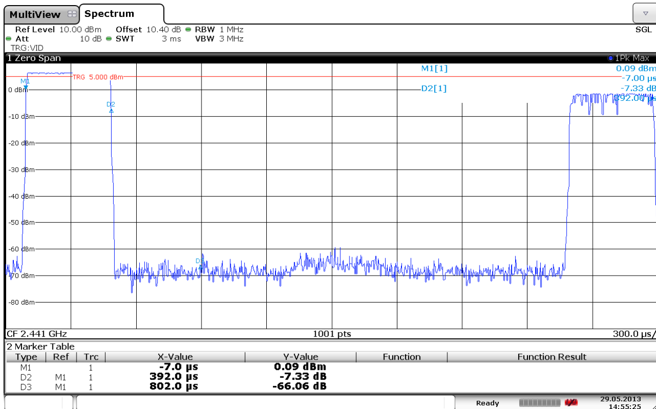
Dwell Time DH1, Hopping Ch 28 - 47
