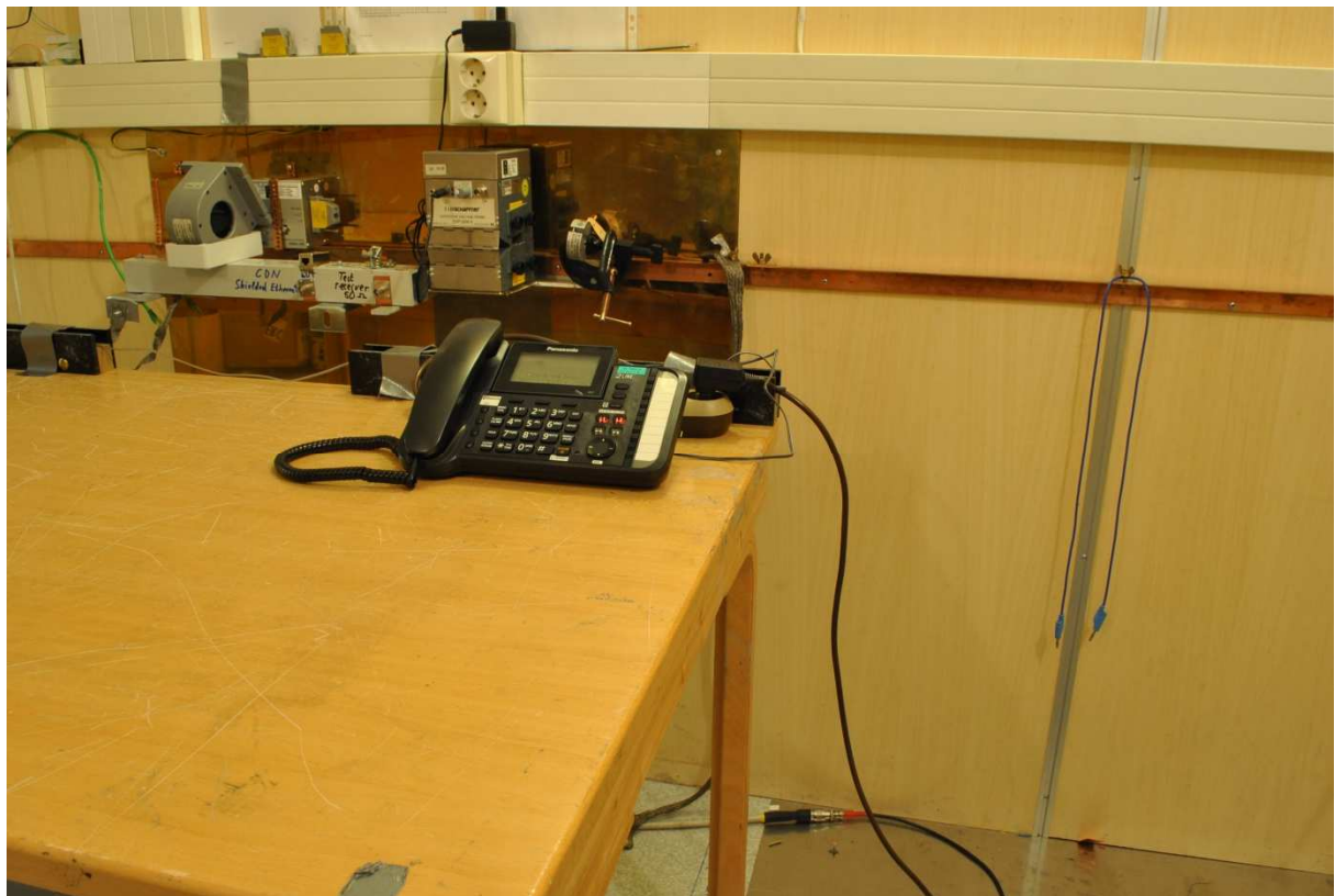
Power-line Conducted Emissions, 120Vac, 60Hz
