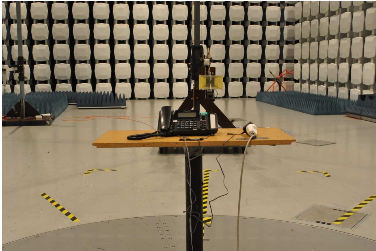
Radiated Emissions, 1 – 25 GHz, 3 meter & 1 meter
