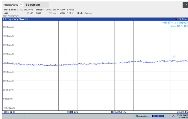
Pre-scan 18 - 26 GHz, 2441 MHz, GFSK, @approx. 10cm
