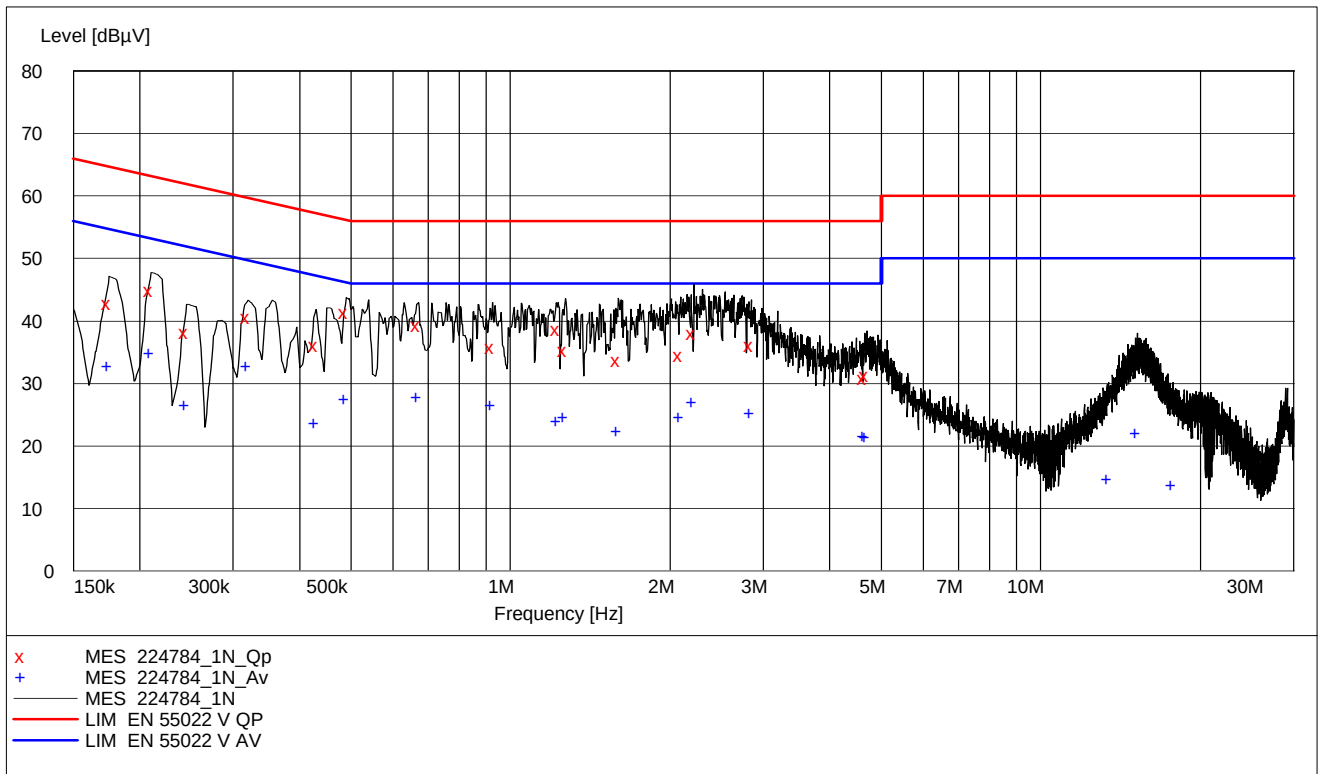
PNLV233 (UC), Charging (Plot shows worst case of Phase L1 and N)
