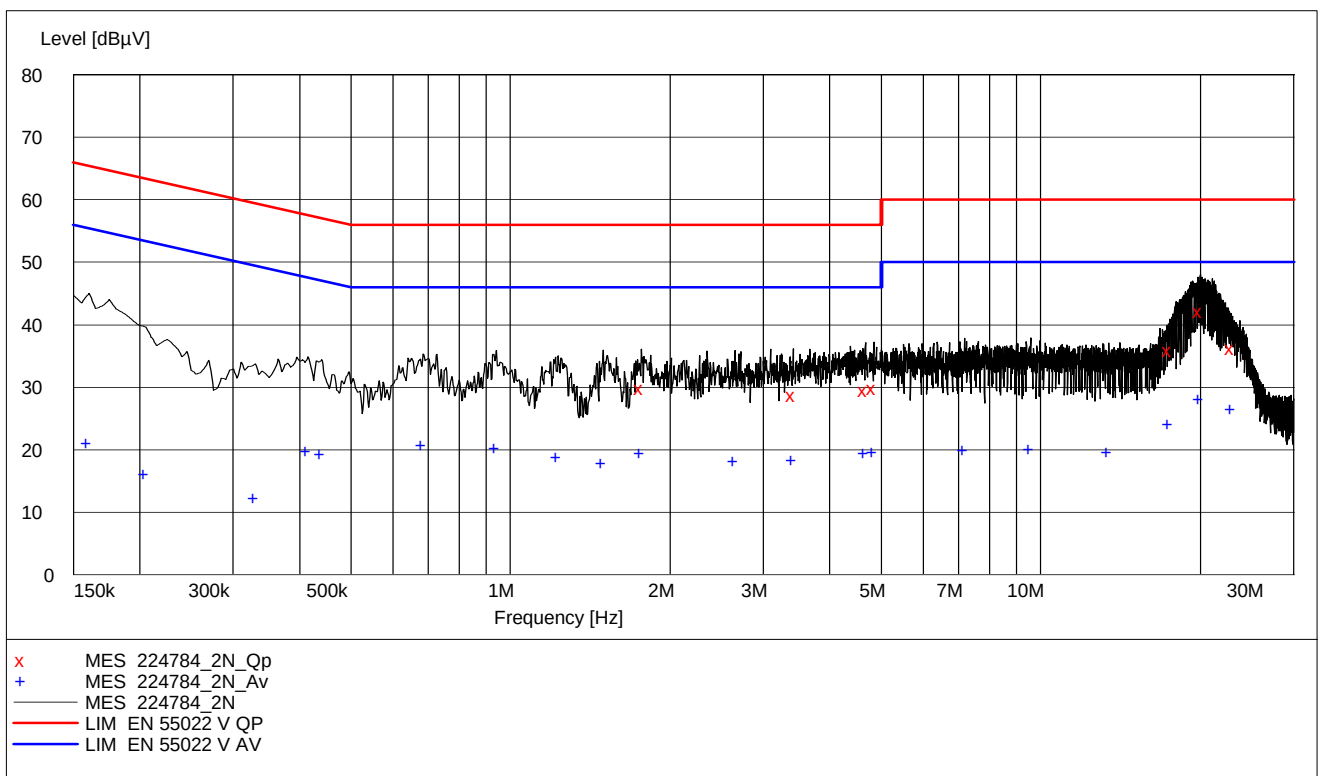
PNLV233 (YJ), Charging (Plot shows worst case of Phase L1 and N)
