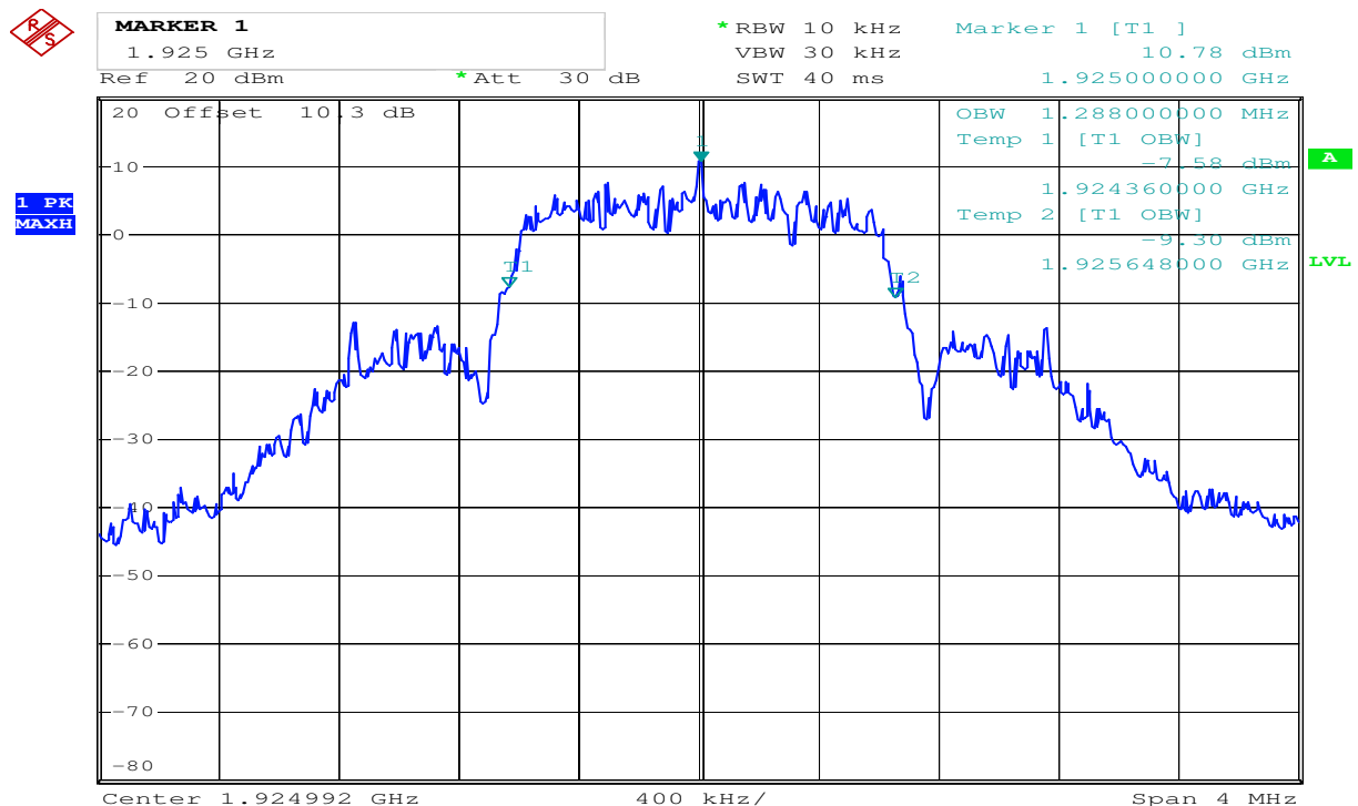
Emission Bandwidth B , Middle Channel
