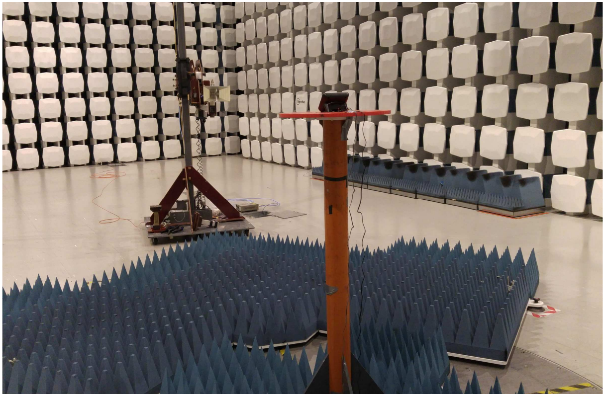
Radiated Emissions, 1 GHz - 8.5 GHz
