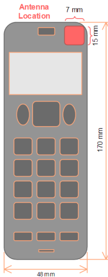
Fig. 1: Antenna location of the EUT.
