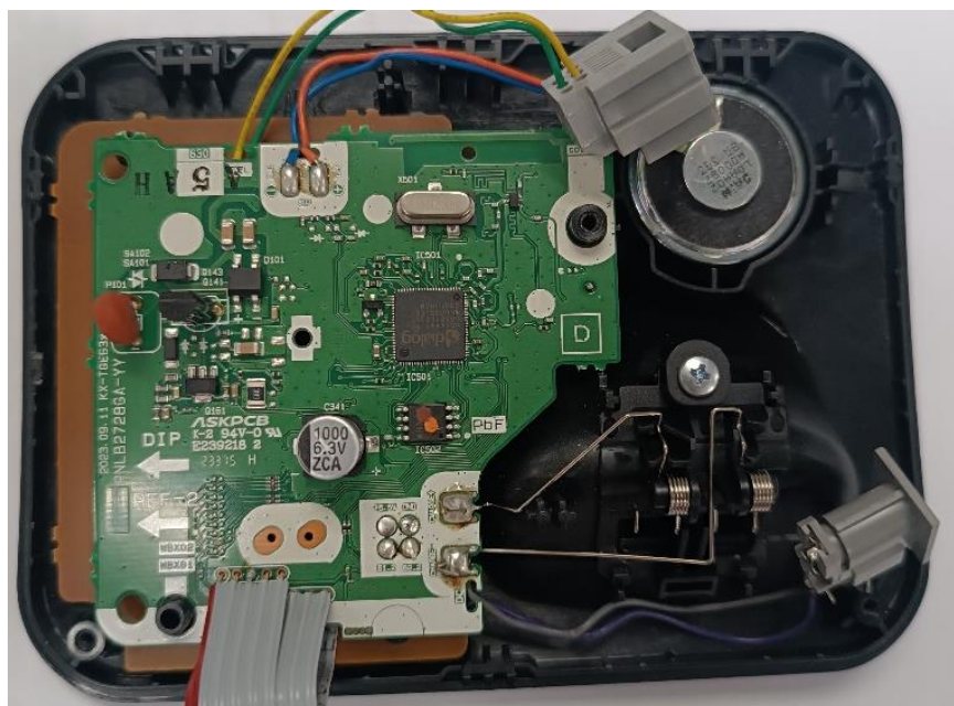
Internal View KX-TGE630
