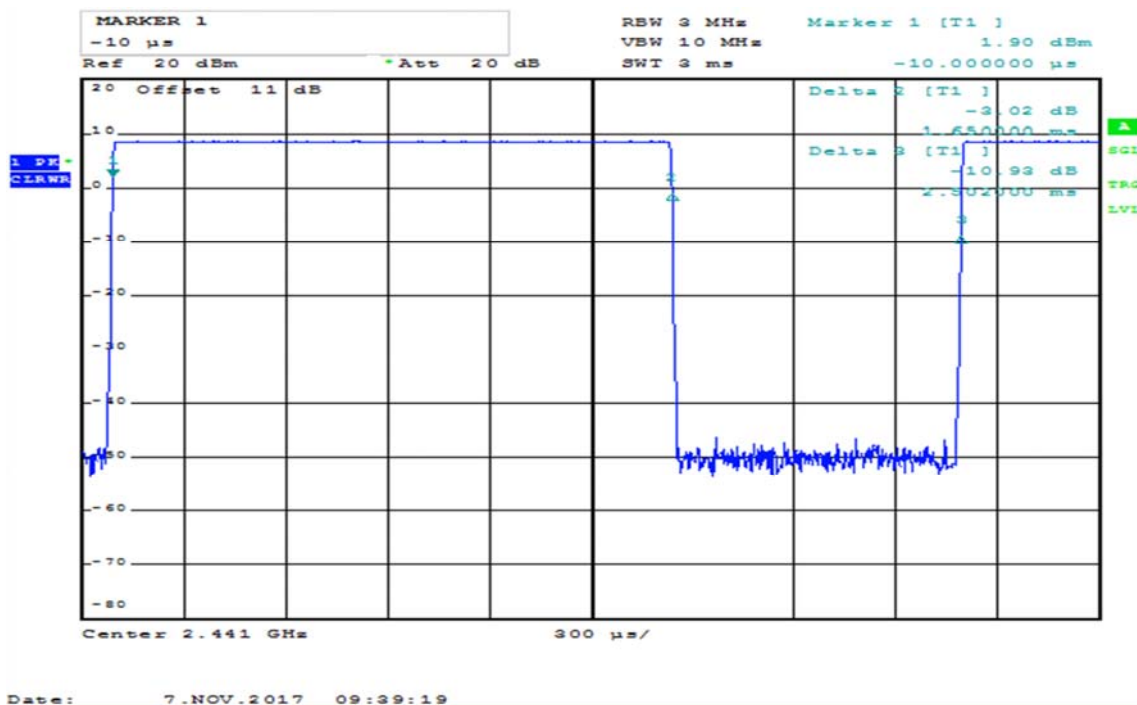
Burst Length DH3
