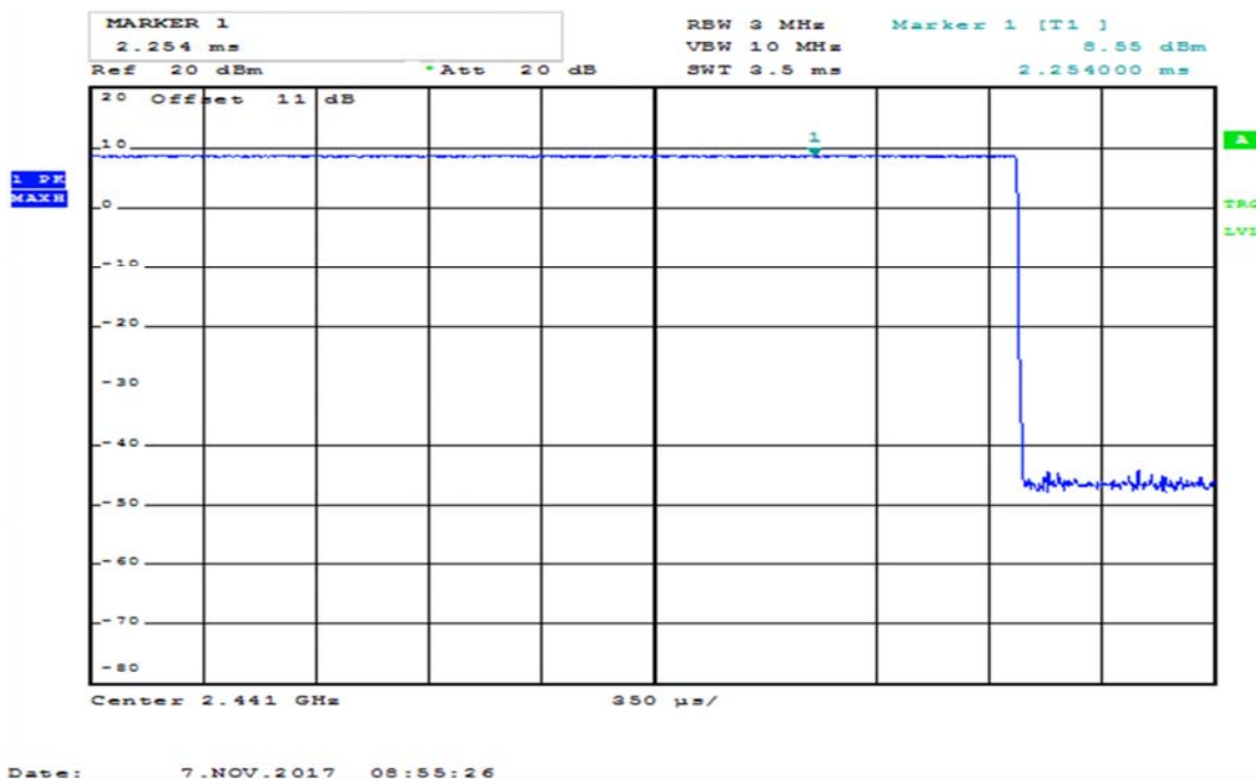
Conducted Power, 2441 MHz
