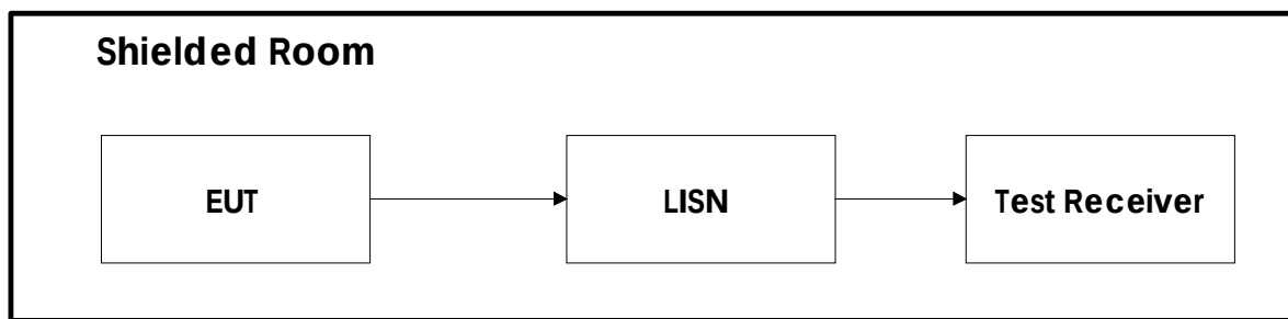
Test Set-Up 5
