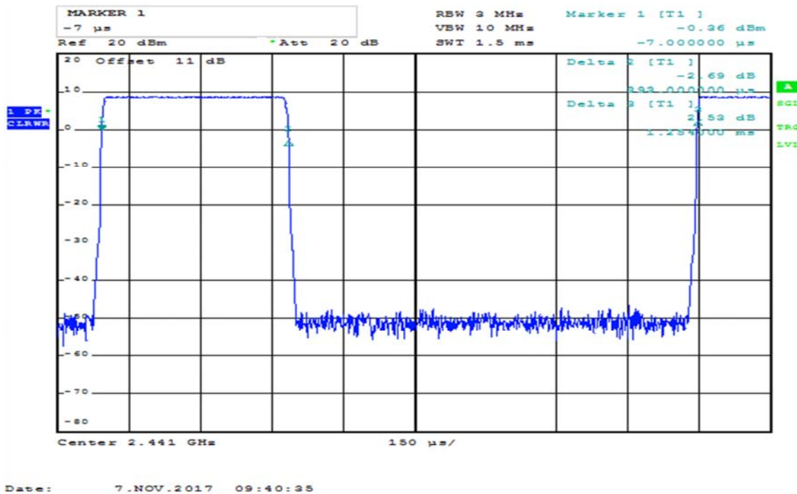
Burst Length DH1
