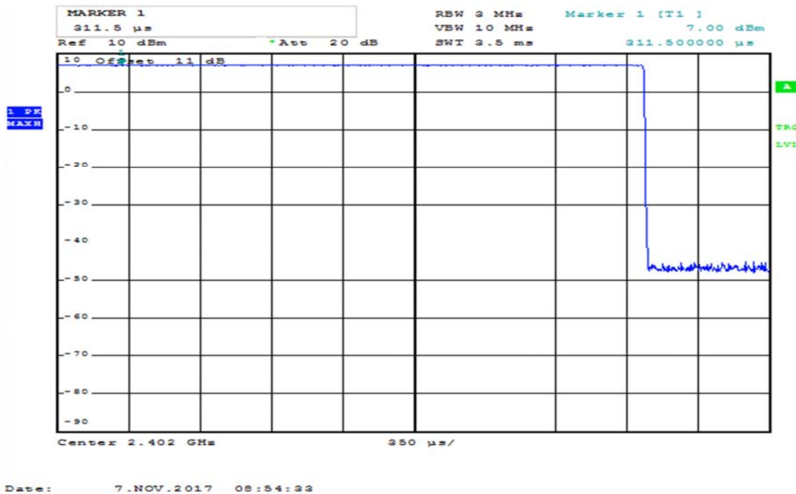
Conducted Power, 2402 MHz
