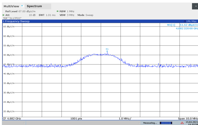
Radiated Emissions 4882 MHz, 2441 MHz, GFSK, Peak (Max: VP)
