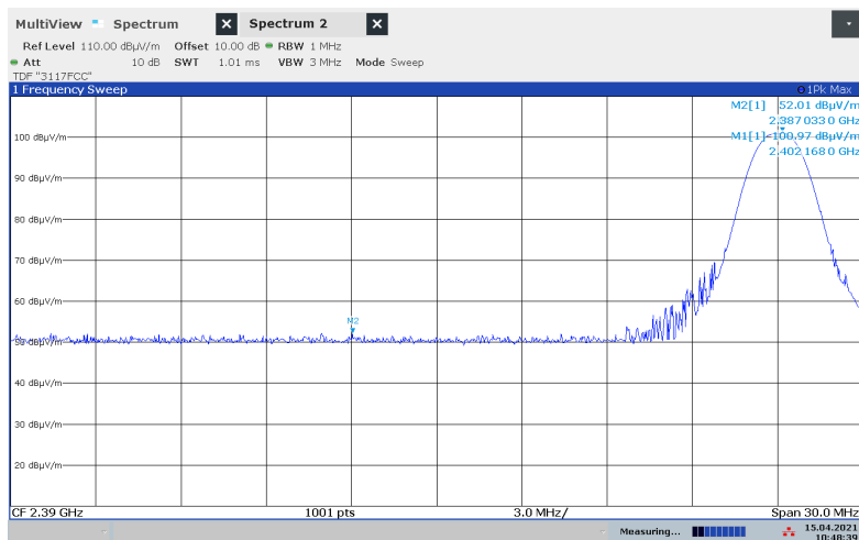
Lower Band Edge 2402 MHz, GFSK, Peak
