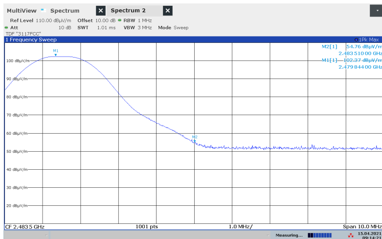
Upper Band Edge 2480 MHz, GFSK, Peak
