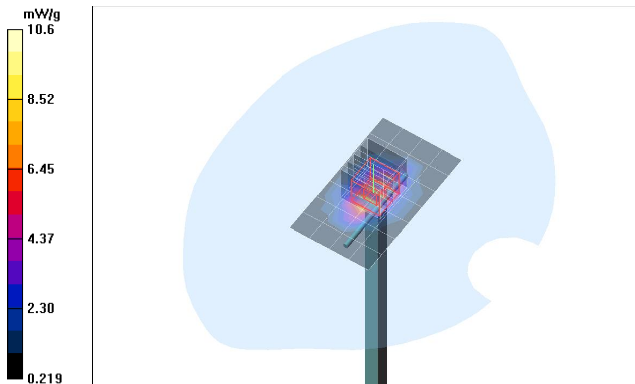
Plot. 3: System Verification Measurement 1900 MHz, Head.
