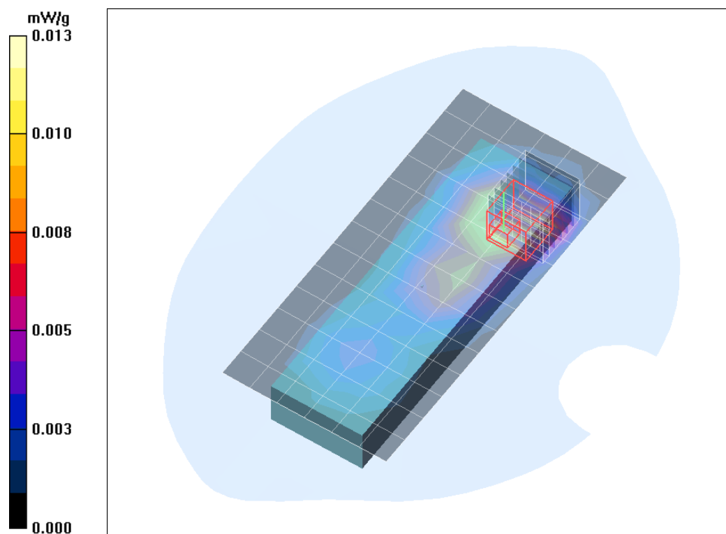
Plot. 2: SAR distribution plot for DECT, channel 4, body-worn configuration, front side, 0mm distance to phantom.
