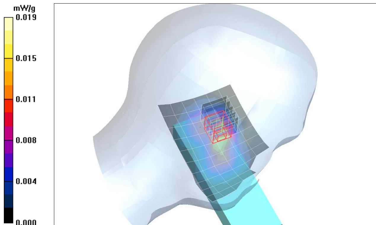
Plot. 1: SAR distribution plot for DECT, channel 2, head configuration, left cheek.
