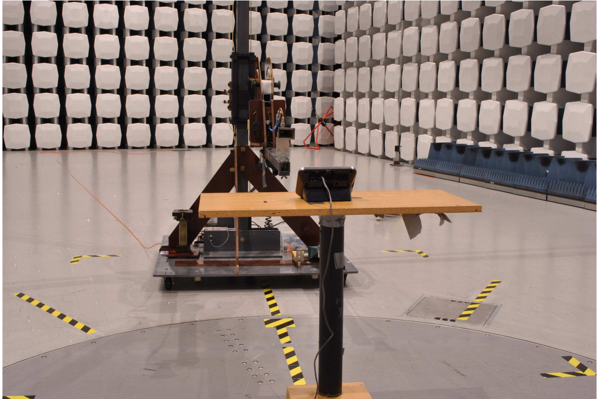
Radiated Emissions Test (Tests were performed on KX-TG7871)
