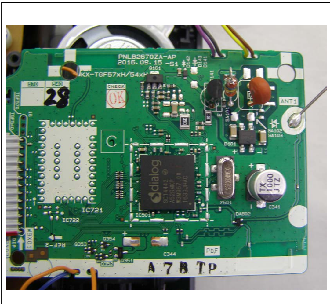
Main Board (RF part)
