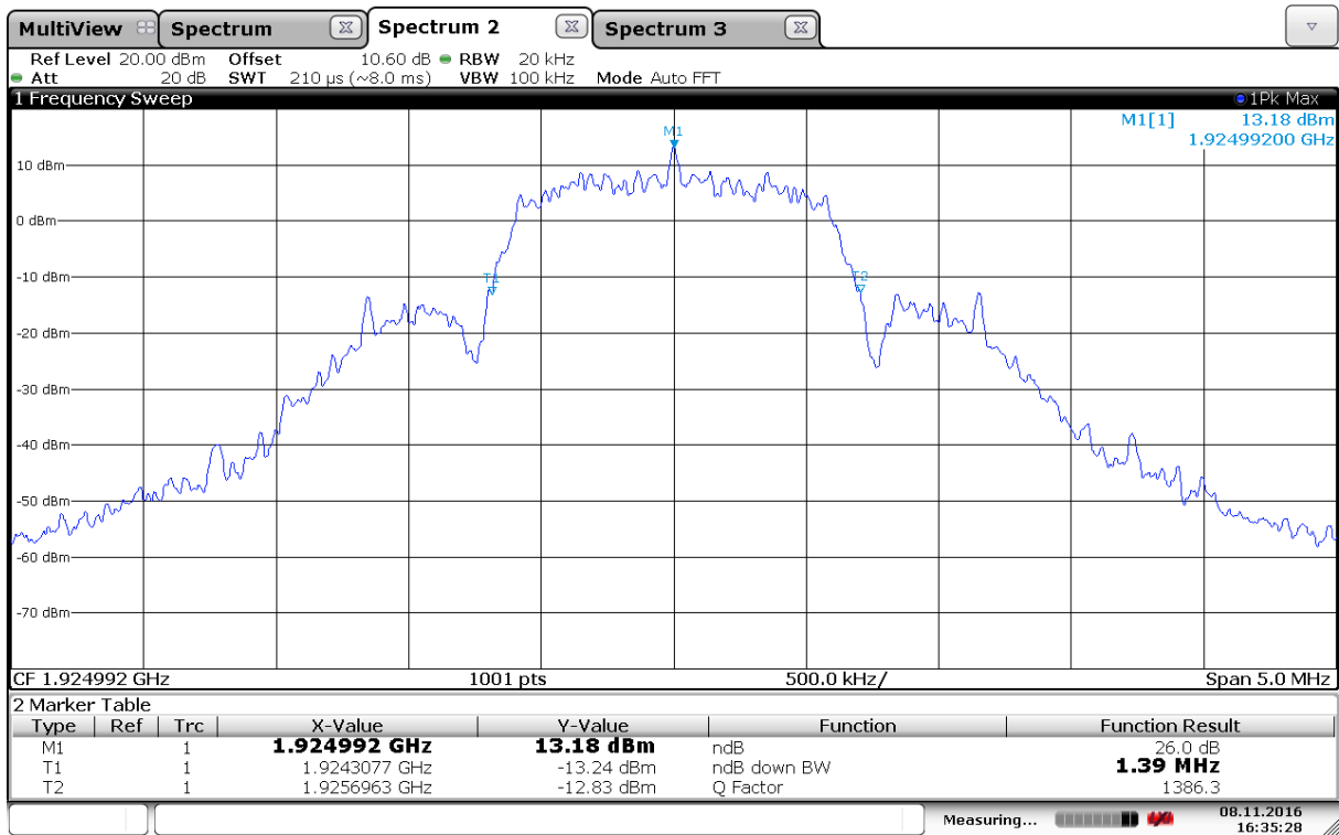
Emission Bandwidth B, Mid Channel
