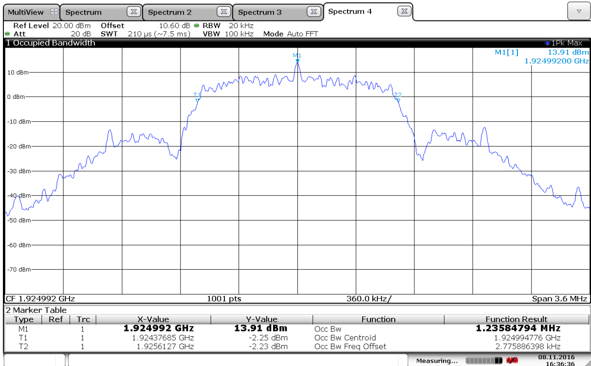
99% Bandwidth, Mid Channel
