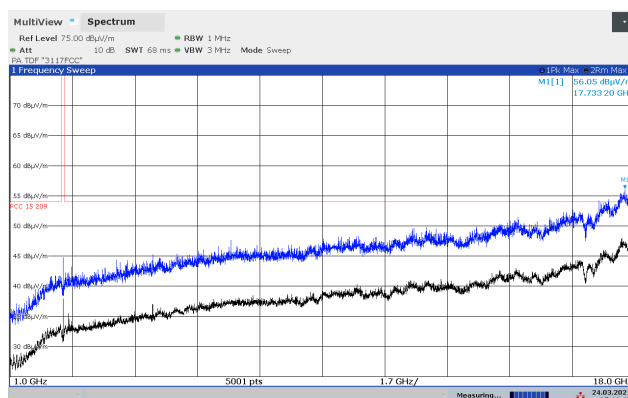
Radiated Emissions 1 - 18 GHz, 2441 MHz, GFSK, VP
