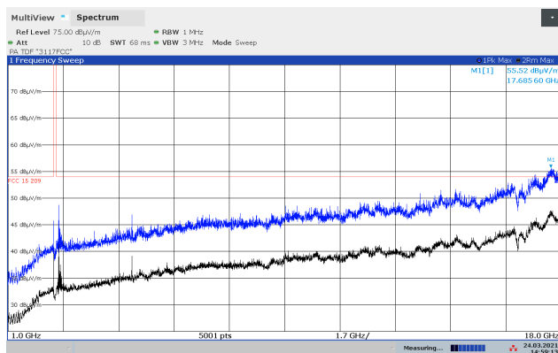
Radiated Emissions 1 - 18 GHz, 2402 MHz, GFSK, HP
