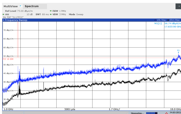
Radiated Emissions 1 - 18 GHz, 2441 MHz, GFSK, HP
