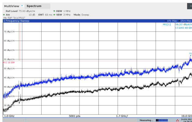
Radiated Emissions 1 - 18 GHz, 2402 MHz, GFSK, VP
