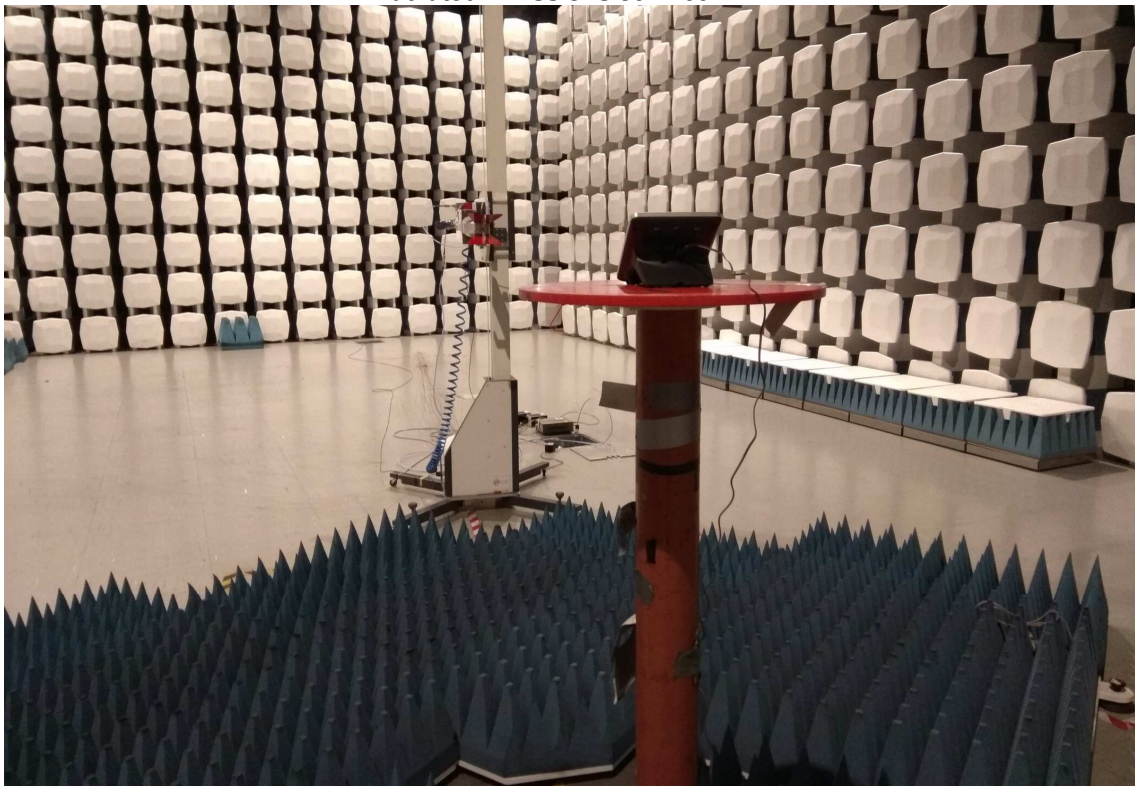
Radiated Emissions 1 GHz – 18 GHz
