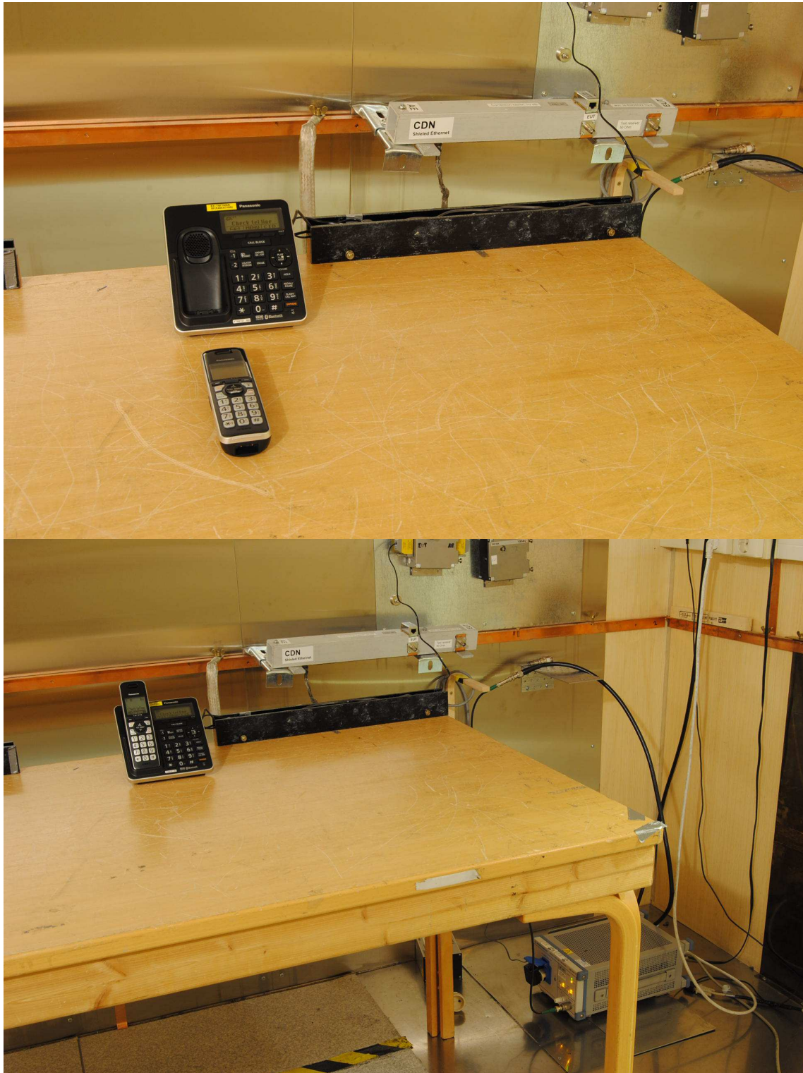
Power-Line Conducted Emissions Test
