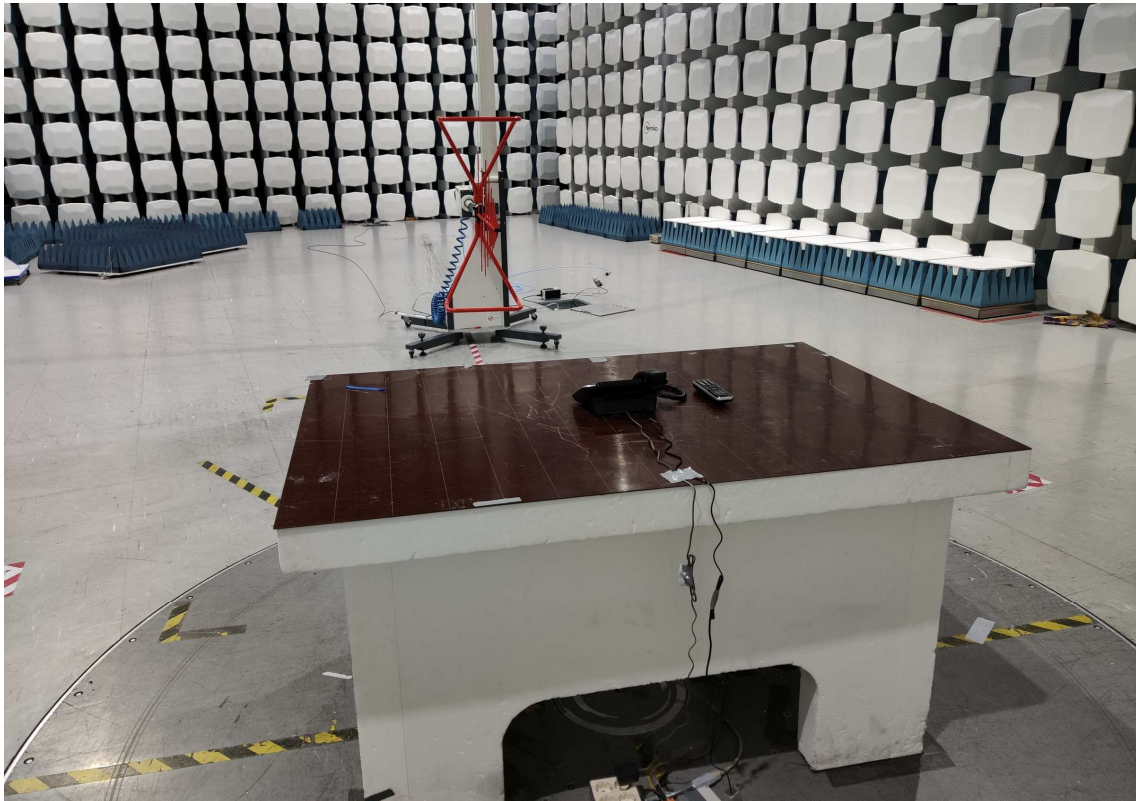
Radiated Emissions 30 - 200 MHz
