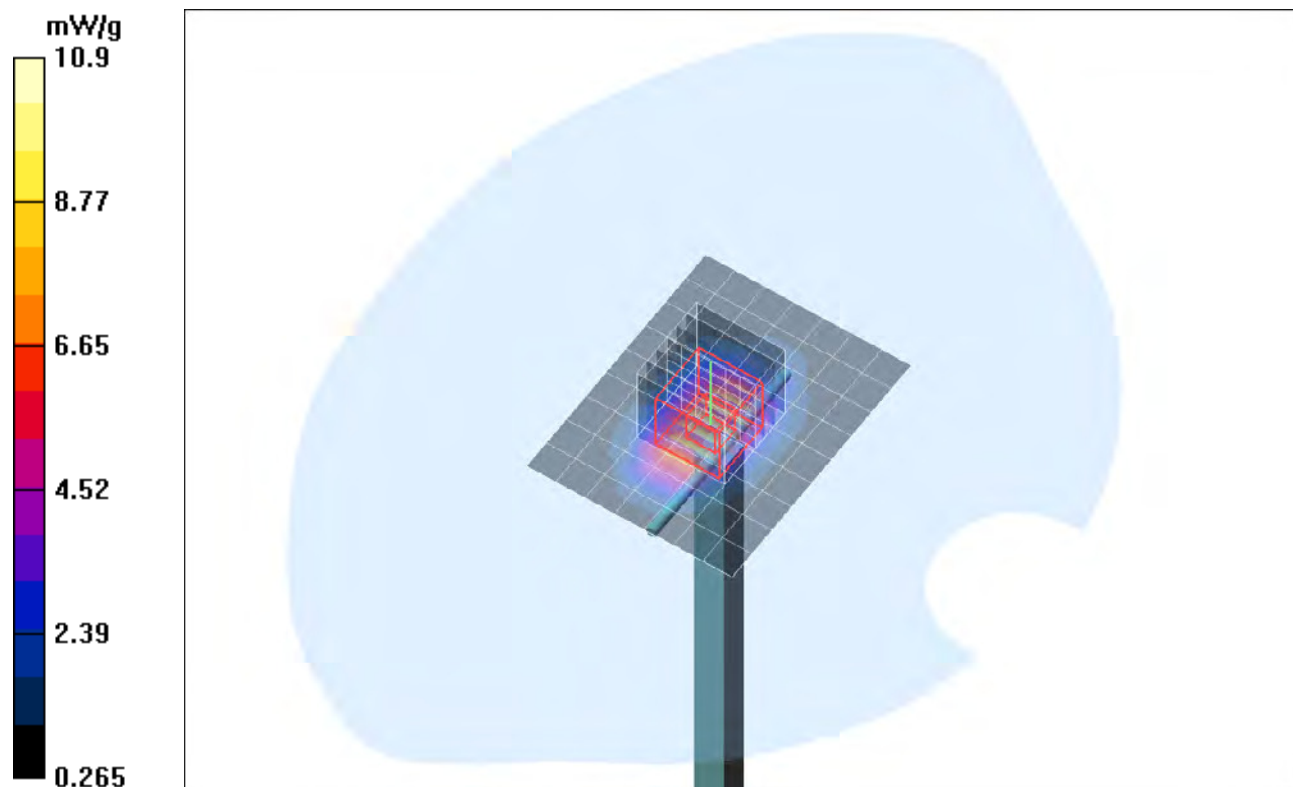
Plot. 12: System Verification measurement 1900 MHz, body.
