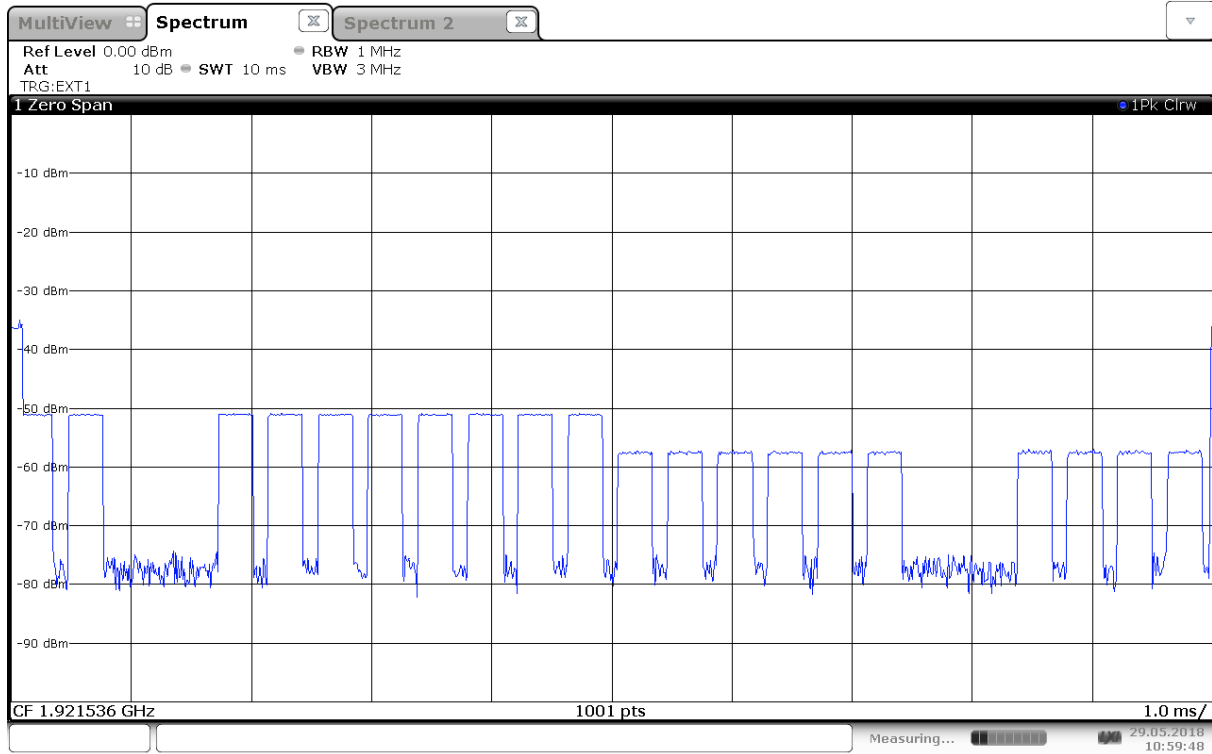
8.3.2c) EUT Transmits on Interference Free RECEIVE Slot, BEFORE, Long Slot
