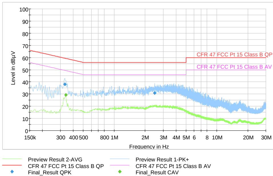
KX-TGU430 Hook-Off, PNLV226 (UC)
