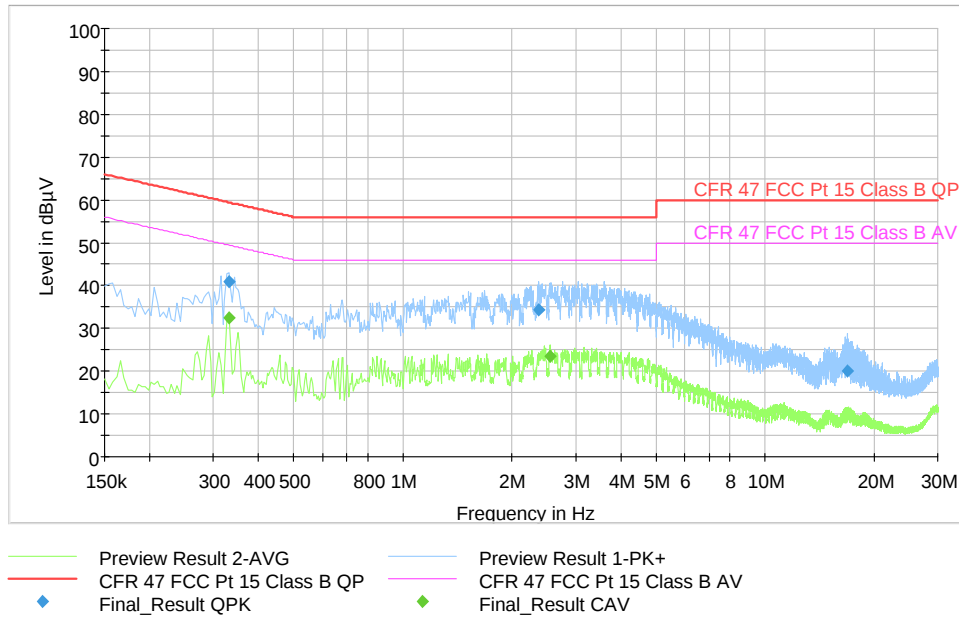
KX-TGU120 Handset Charging, PNLV226 (UC)
