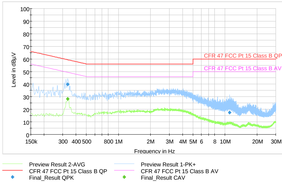
KX-TGU120 Hook-Off, PNLV226 (UC)
