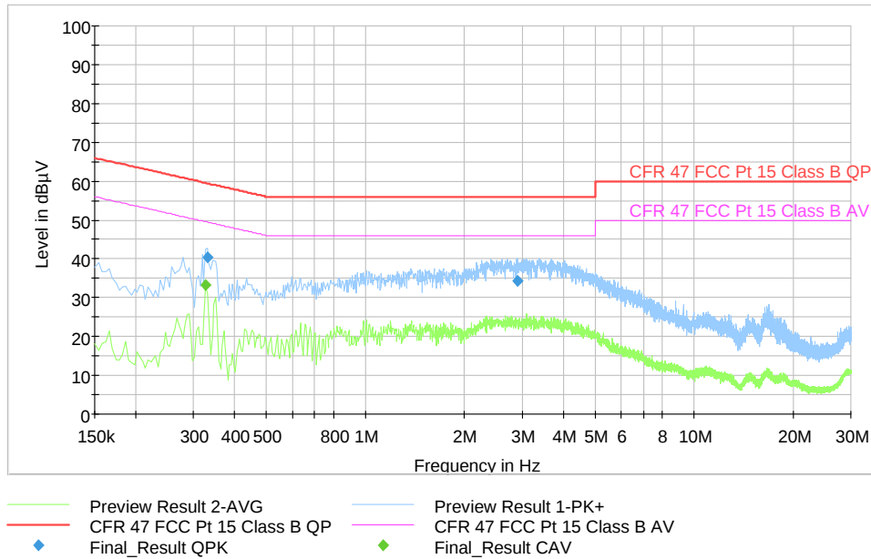
KX-TGU430 Handset Charging, PNLV226 (UC)
