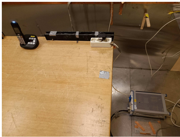
Power-Line Conducted Emissions, KX-TGU430
