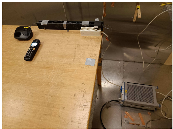
Power-Line Conducted Emissions, KX-TGU120
