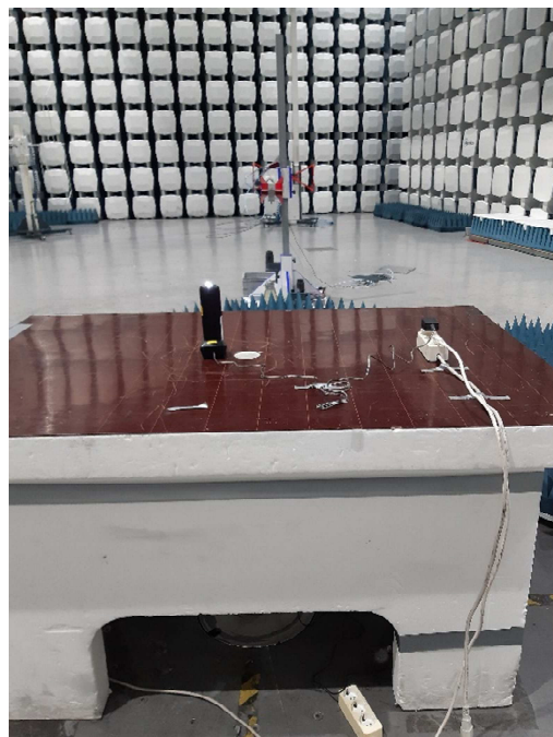
Handset and Charger, On-hook, Radiated emissions
