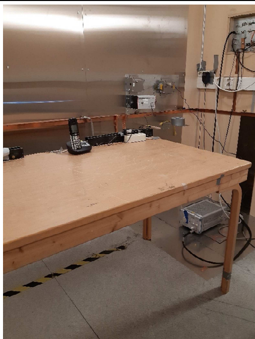
Base and Handset, On-hook, Conducted emissions
