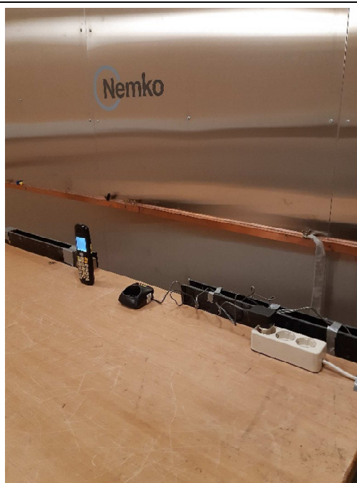
Handset and Charger, Off-hook, Conducted emissions
