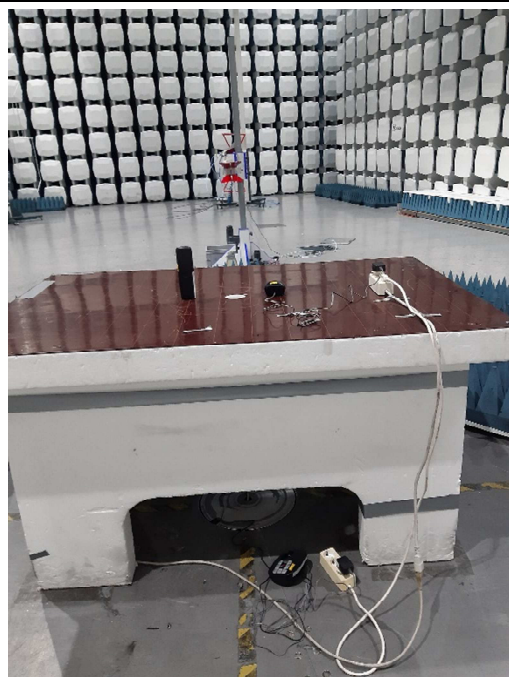
Handset and Charger, Off-hook, Radiated emissions
