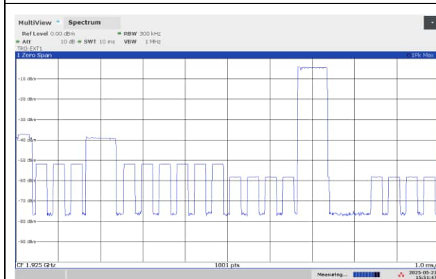
EUT Transmits on Free RECEIVE Slot, AFTER
