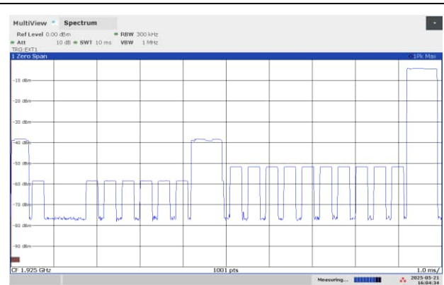
EUT Transmits on Free TRANSMIT Slot, AFTER
