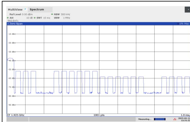
EUT Transmits on Free RECEIVE Slot, BEFORE
