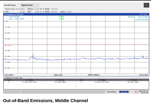
Out-of-Band Emissions, Middle Channel
