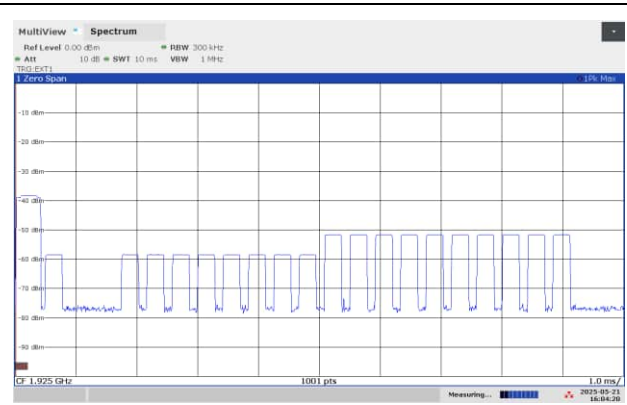
EUT Transmits on Free TRANSMIT Slot, BEFORE
