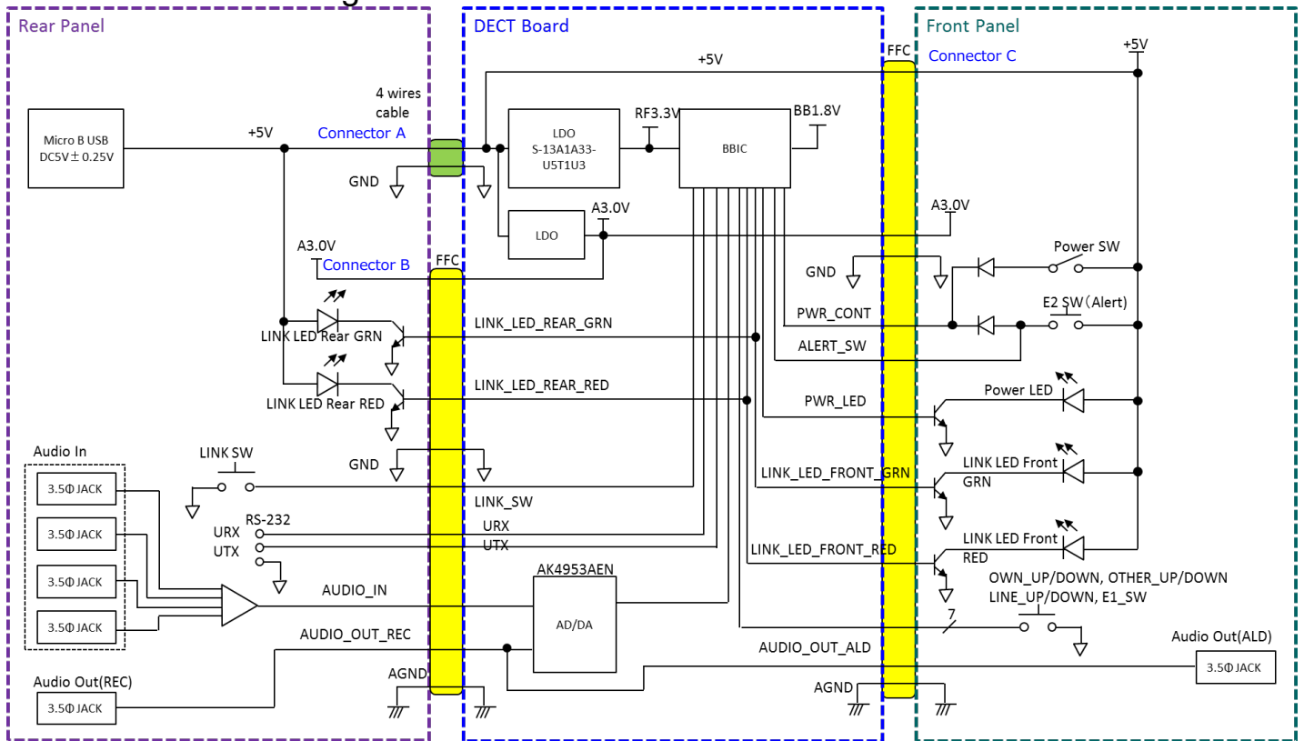
ConnectorA B4B-ZR-SM4-TF(LF)(SN)
