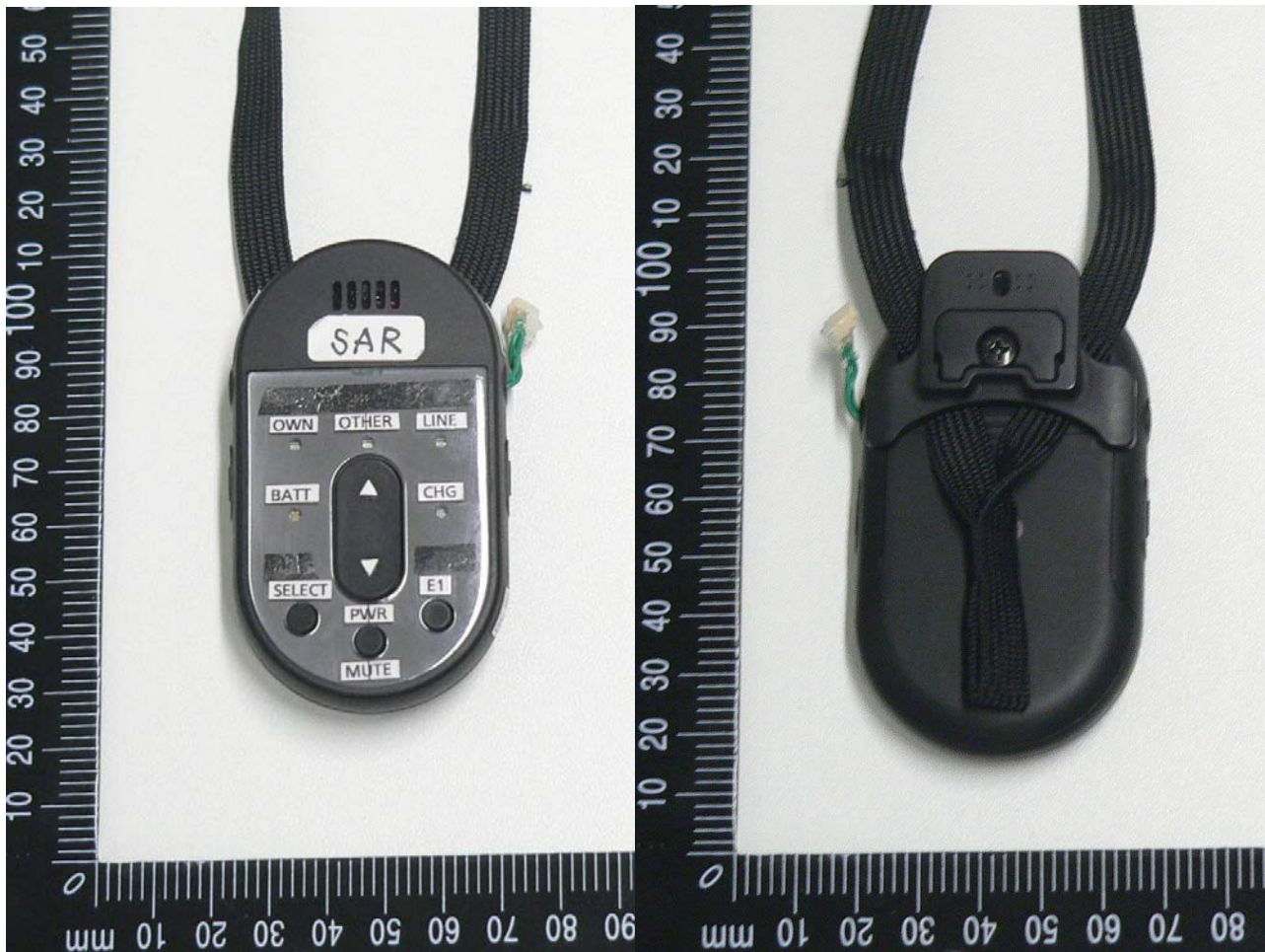
Fig. 7: Front and back view of the device under test.
