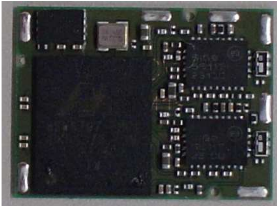
RF Part Module with shield cover removed
