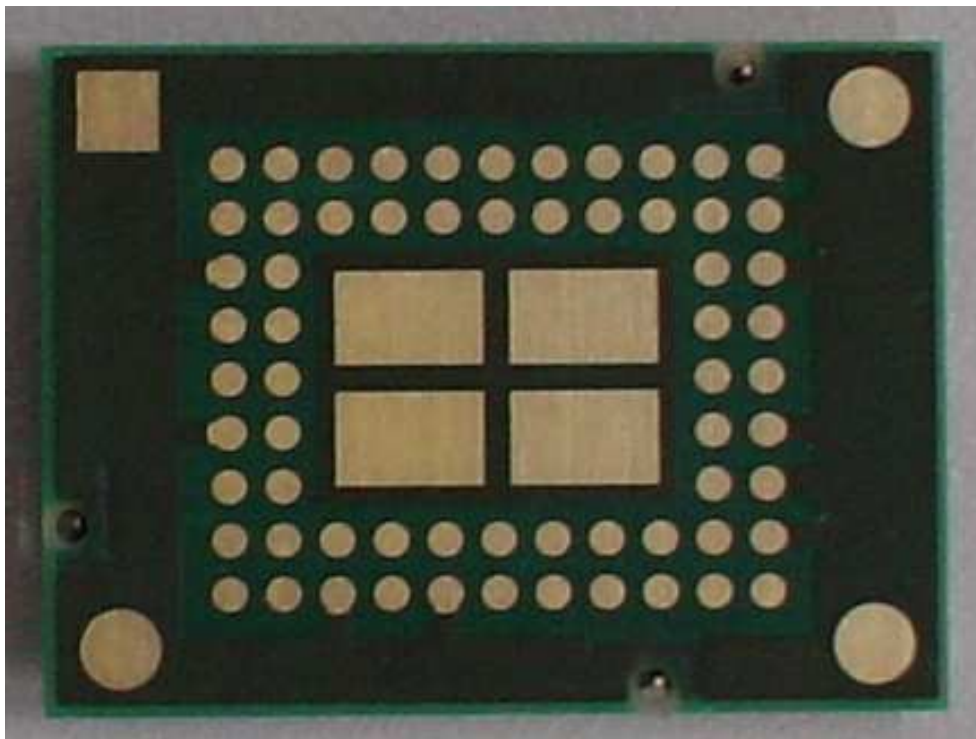
RF Part Module/ Bottom View
