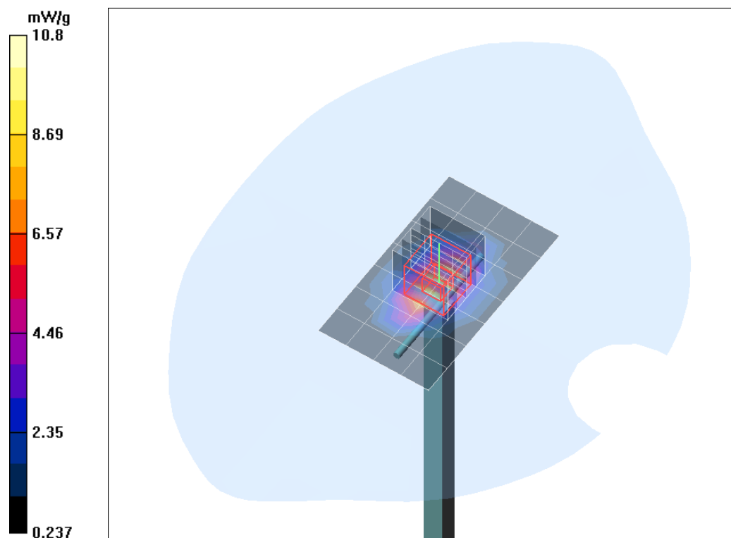
Plot. 2: System Verification Measurement 1900 MHz, Head.
