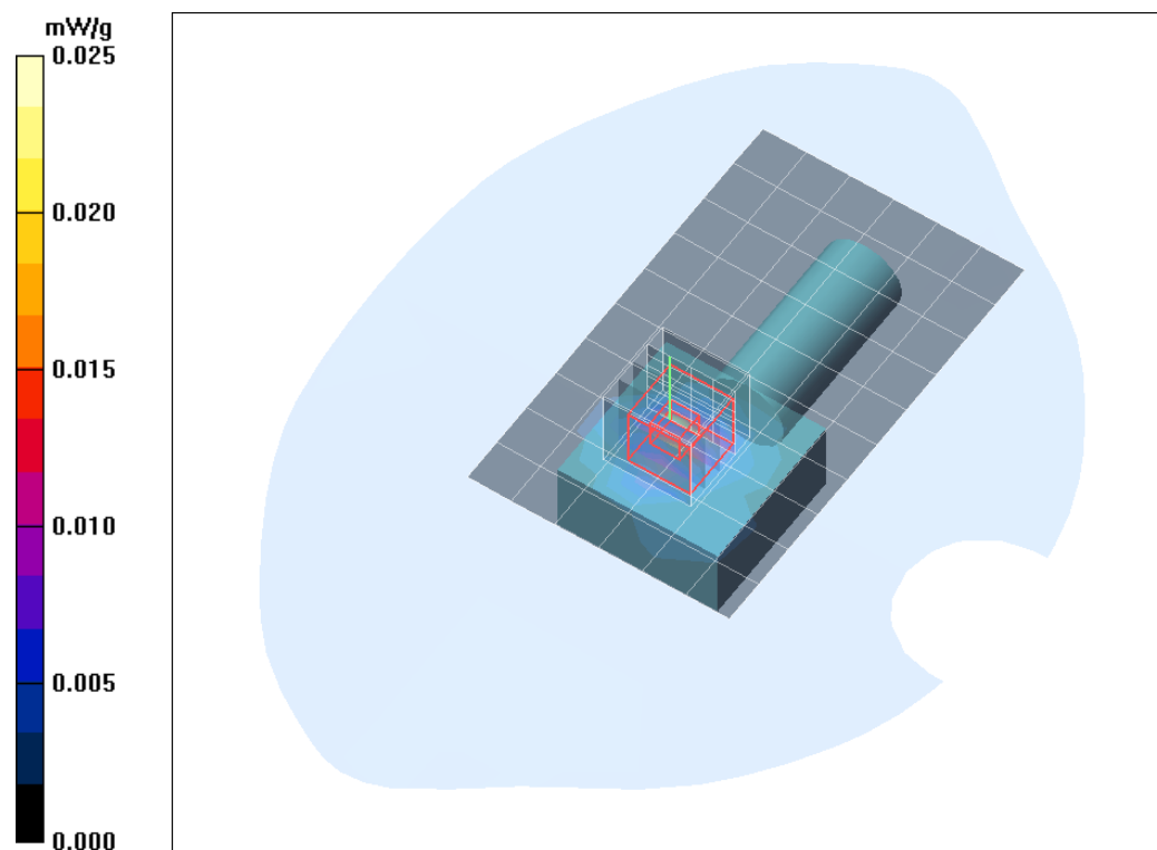
Plot. 1: SAR distribution plot for DECT, channel 2, flat part of the phantom.
