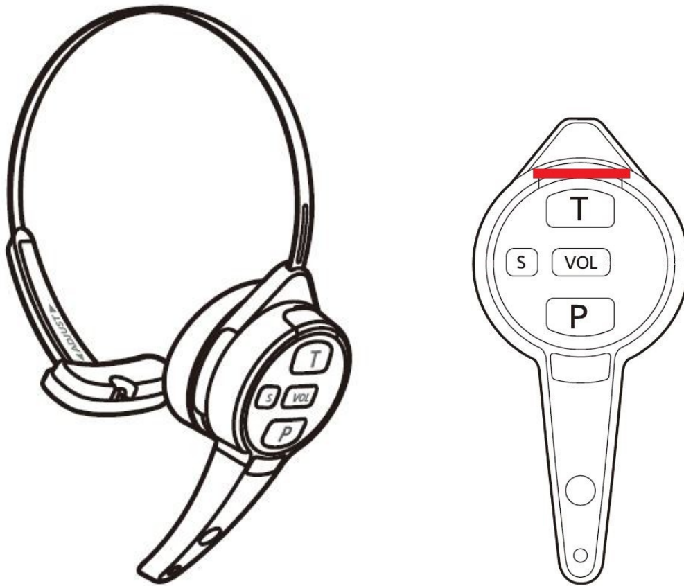
Fig. 1: Sketches and antenna location of the EUT (marked in red).
