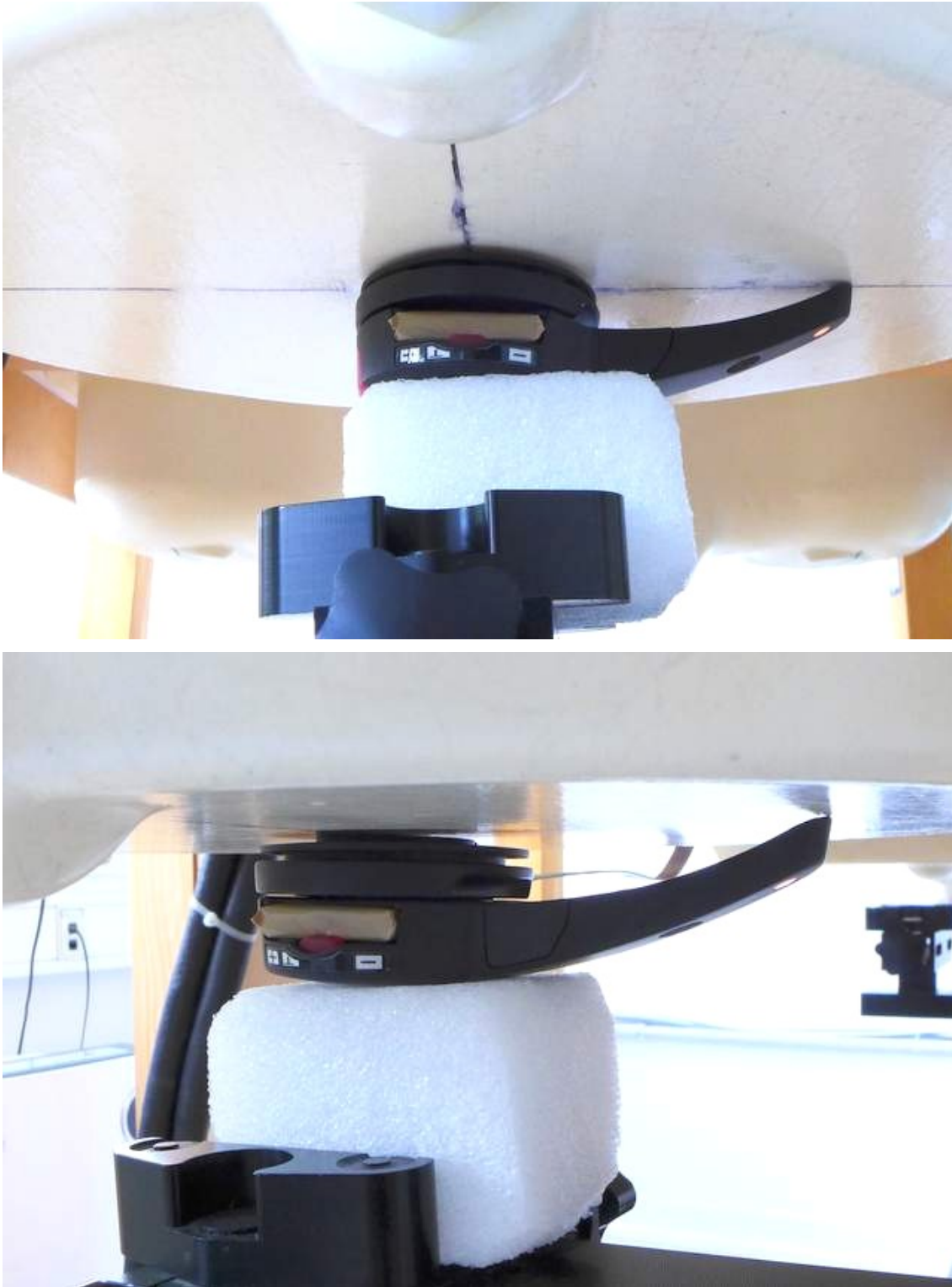
Pic. 3: Test position – inner side, 0mm distance to phantom.
