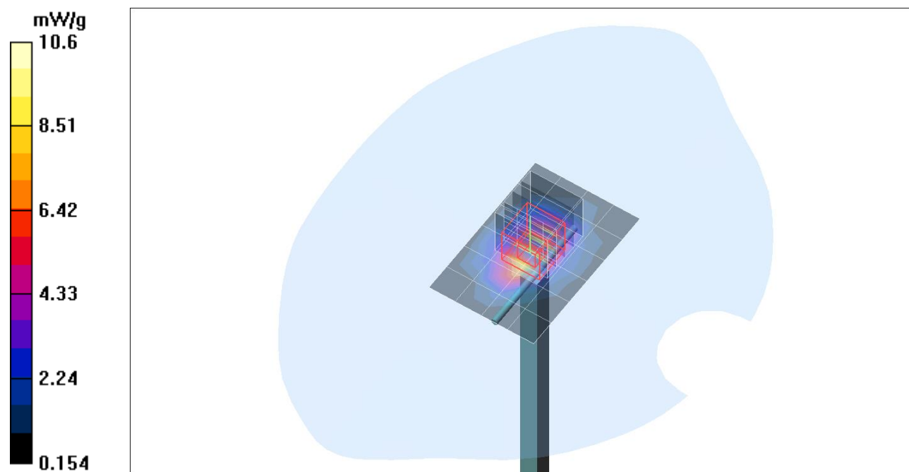
Plot. 3: System Verification Measurement 1900 MHz
