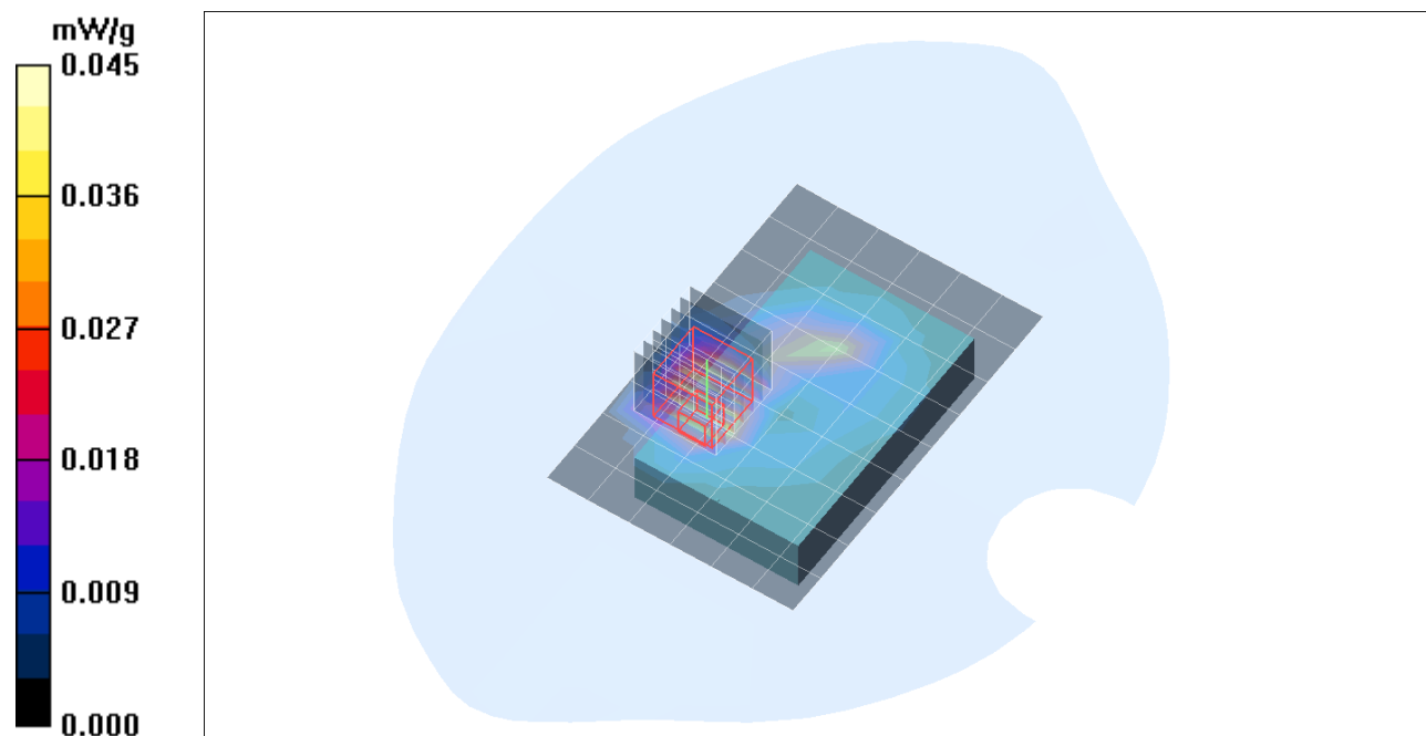
Plot. 1: SAR distribution plot for position 1, front of the DUT towards the phantom, channel 02, antenna 1.
