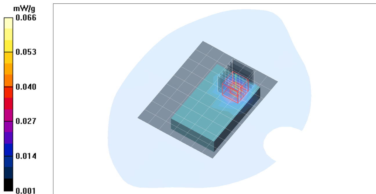
Plot. 2: SAR distribution plot for position 2, back of the DUT towards the phantom, channel 02, antenna 2.
