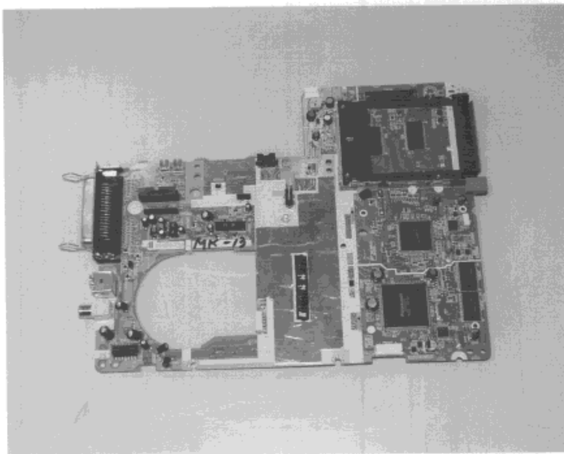
PV-PD2100 Main PCB -2
