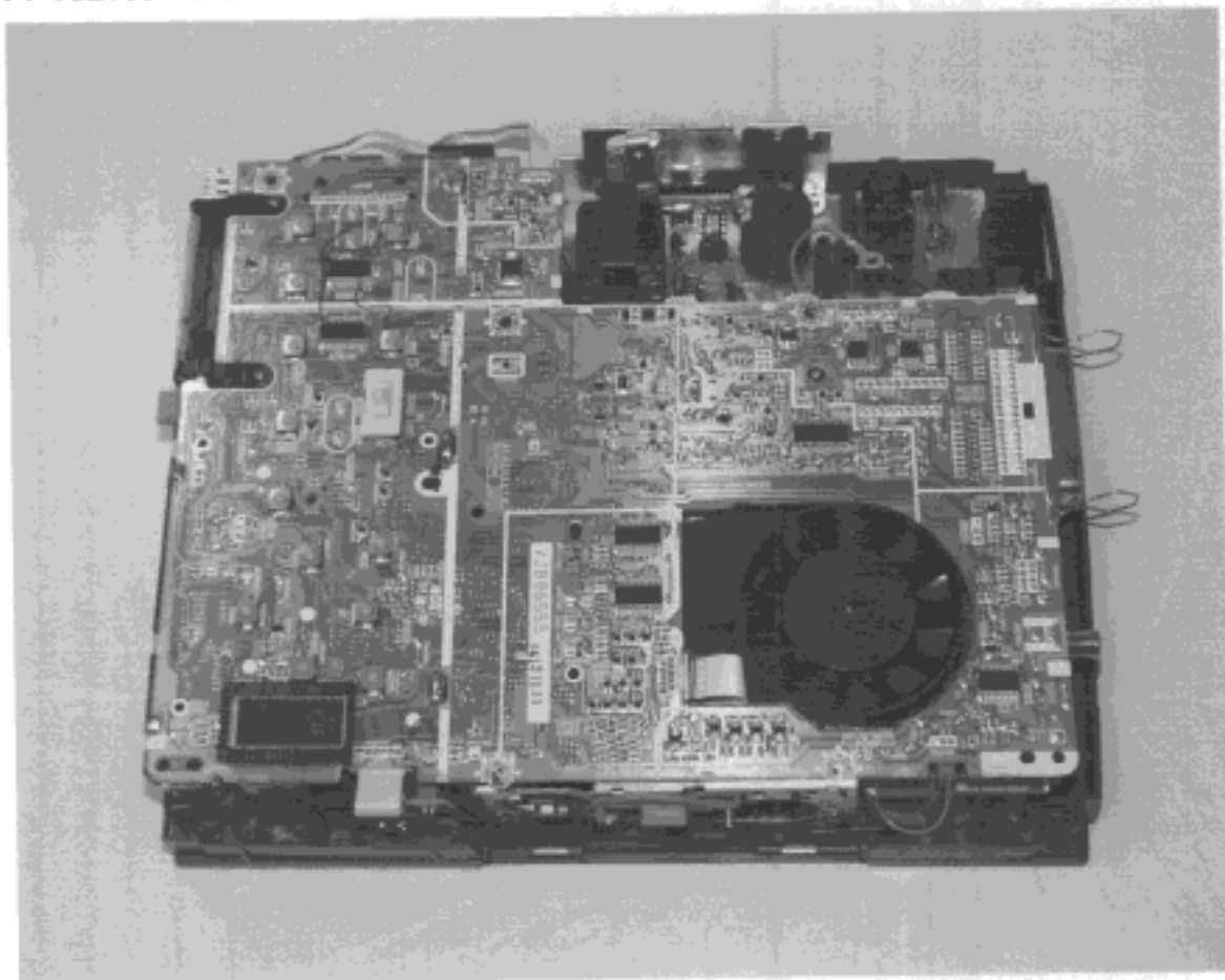
PV-PD2100 Inside View -3
