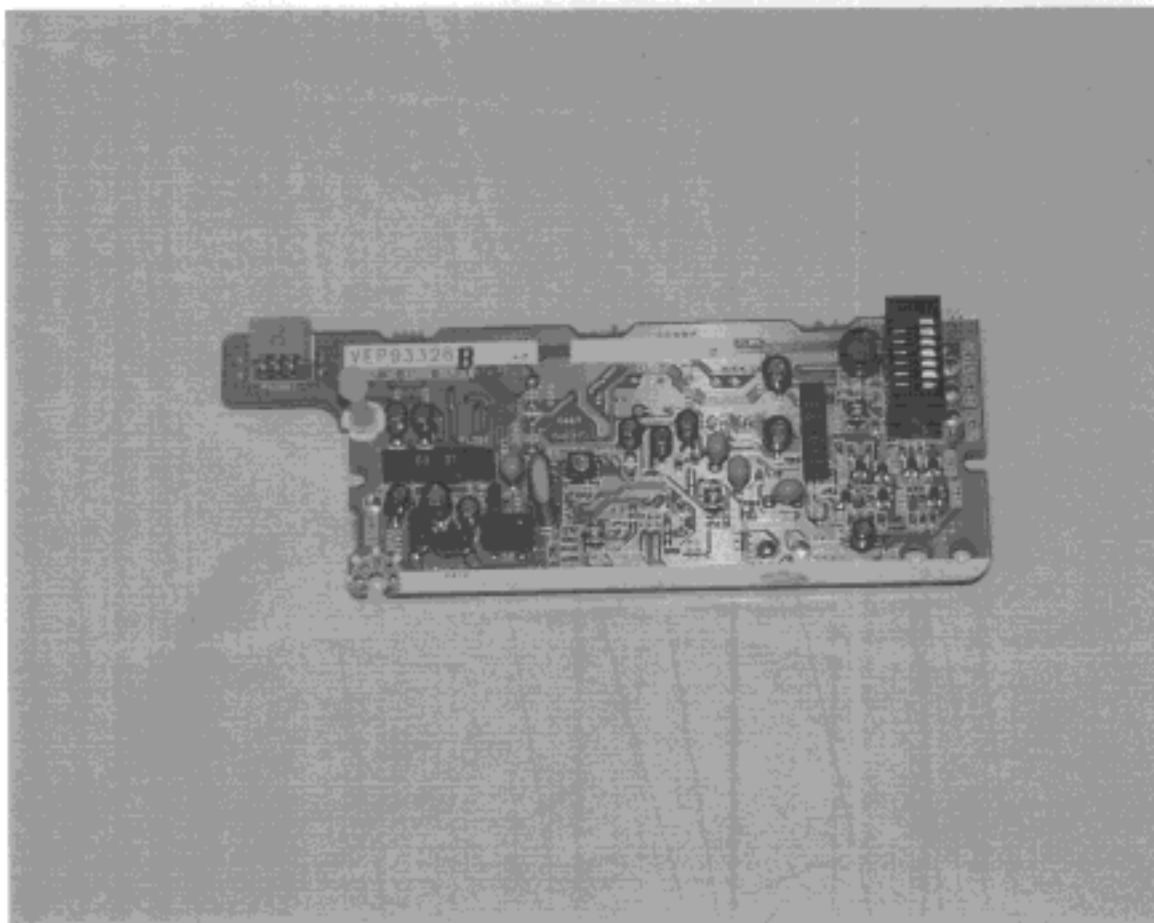
PV-PD2100 Analogr PCB -2
