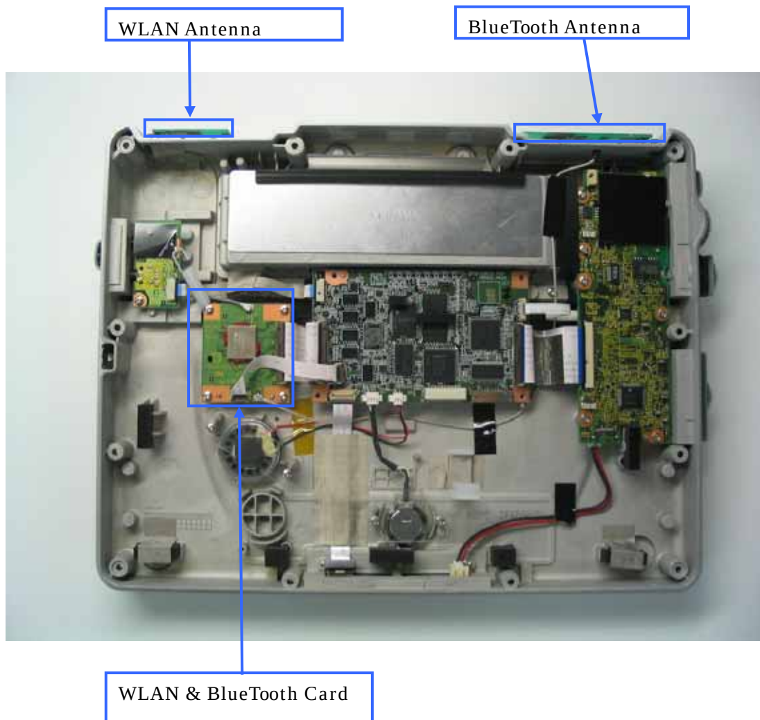
Inside View
