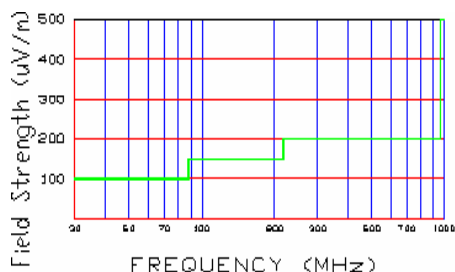
Figure 6-5. Radiated limits at 3 meters.
