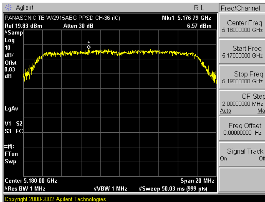
Plot A-8. Peak Power Spectral Density Plot – Low Channel / Low Band (IC)
