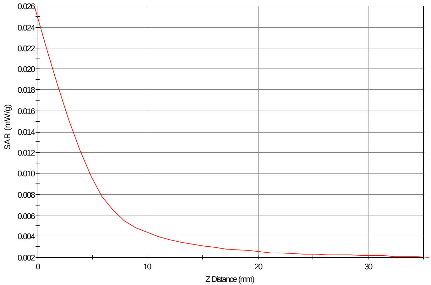
SAR - Z Axis at Hotspot x:44.0 y:-18.0
