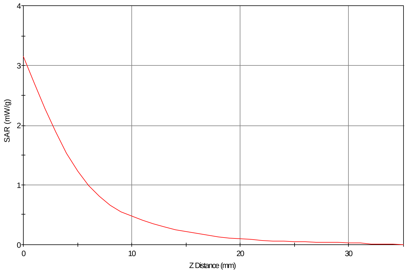
SAR - Z Axis at Hotspot x:77.0 y:-3.0
