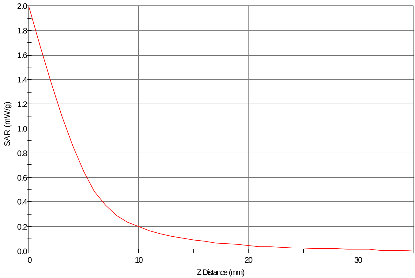
SAR - Z Axis at Hotspot x:43.0 y:12.0
