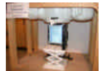
Figure 14.8 Body SAR Test Setup -- 802.11b, Bystander, LCD Open--
