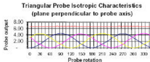
Figure 3.3 Probe Characteristics
