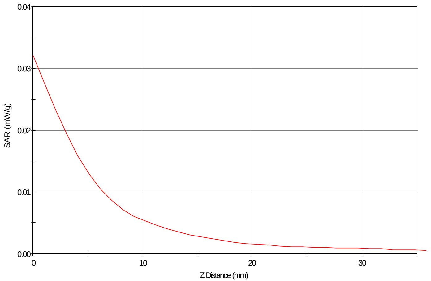
SAR - Z Axis at Hotspot x:-20.0 y:-27.0
