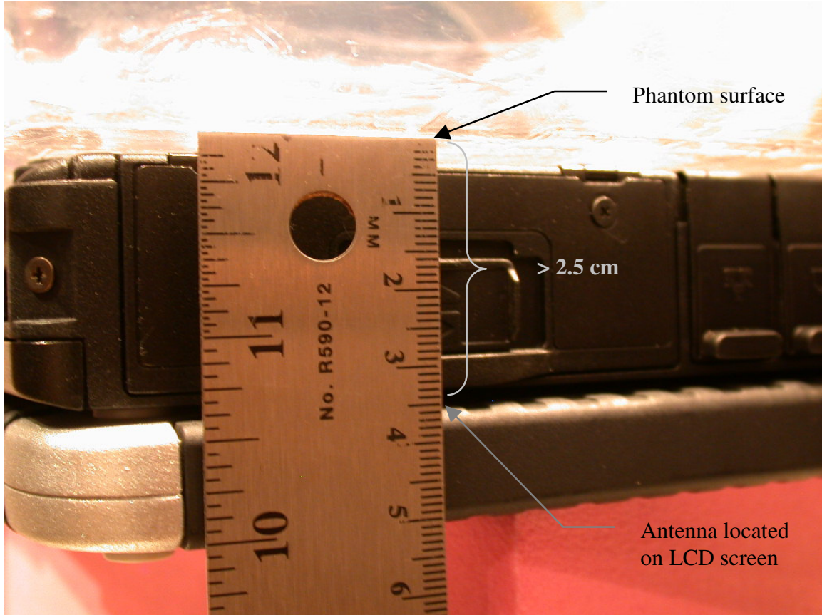
CF-18 WLAN Antenna and Phantom separation distance Illustration
