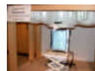
Figure 14.18 Body SAR Test Setup -- 802.11a, Bystander, LCD Flip --
