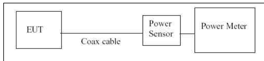
Figure A-2. Test Instrument & Measurement Setup
