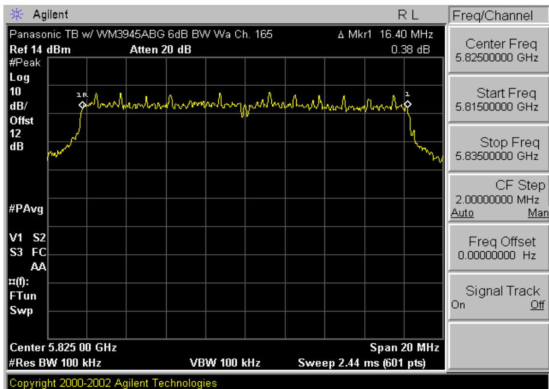
Plot 6-9. 6dB Bandwidth Plot (802.11a – Ch. 165)
