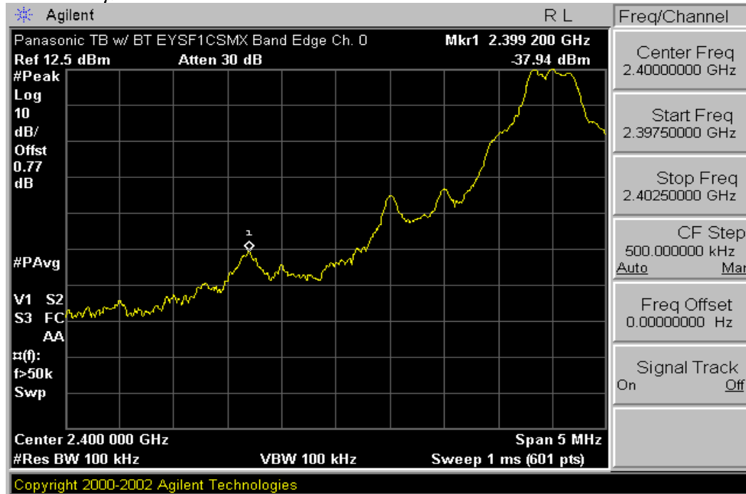
Plot 6-4. Band Edge Plot (Bluetooth – Ch. 0)
