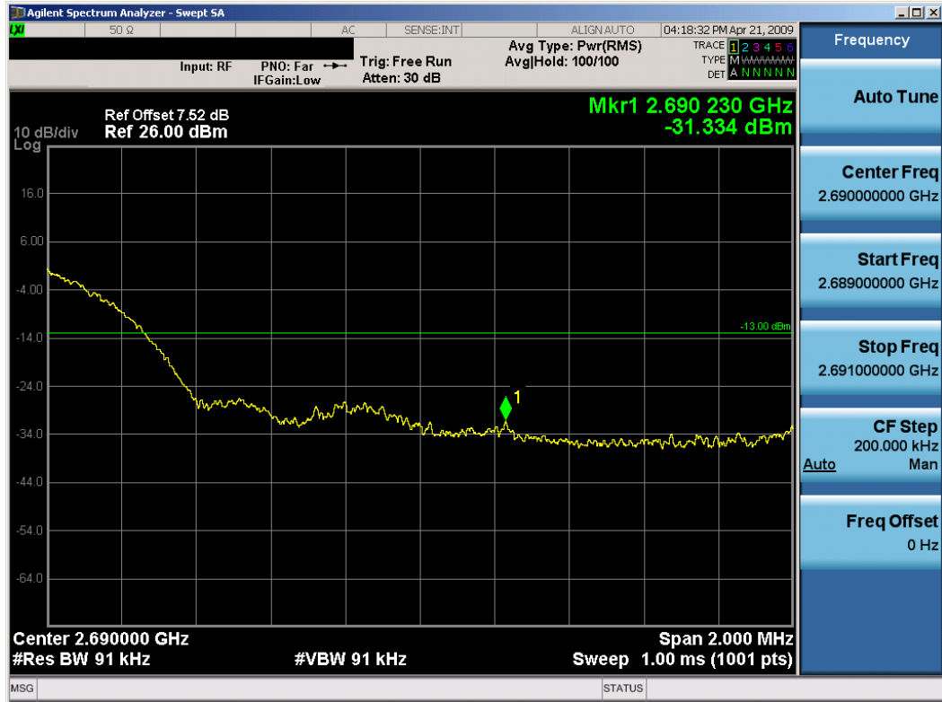
Plot 7-10. Band Edge Plot (TD-CDMA Mode – High Channel)
